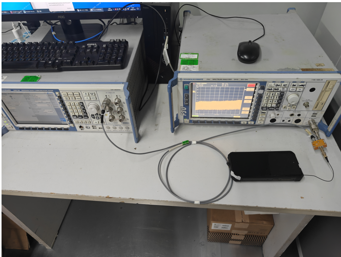
RF Conducted View
