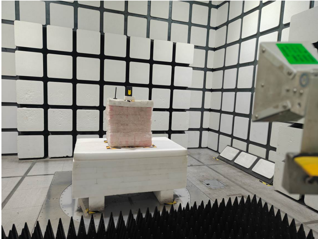
Radiated Emissions View (Above 18 GHz)
