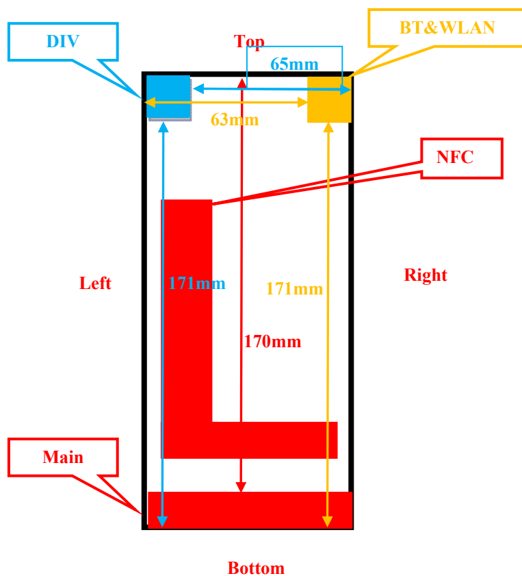
EUT Front View
