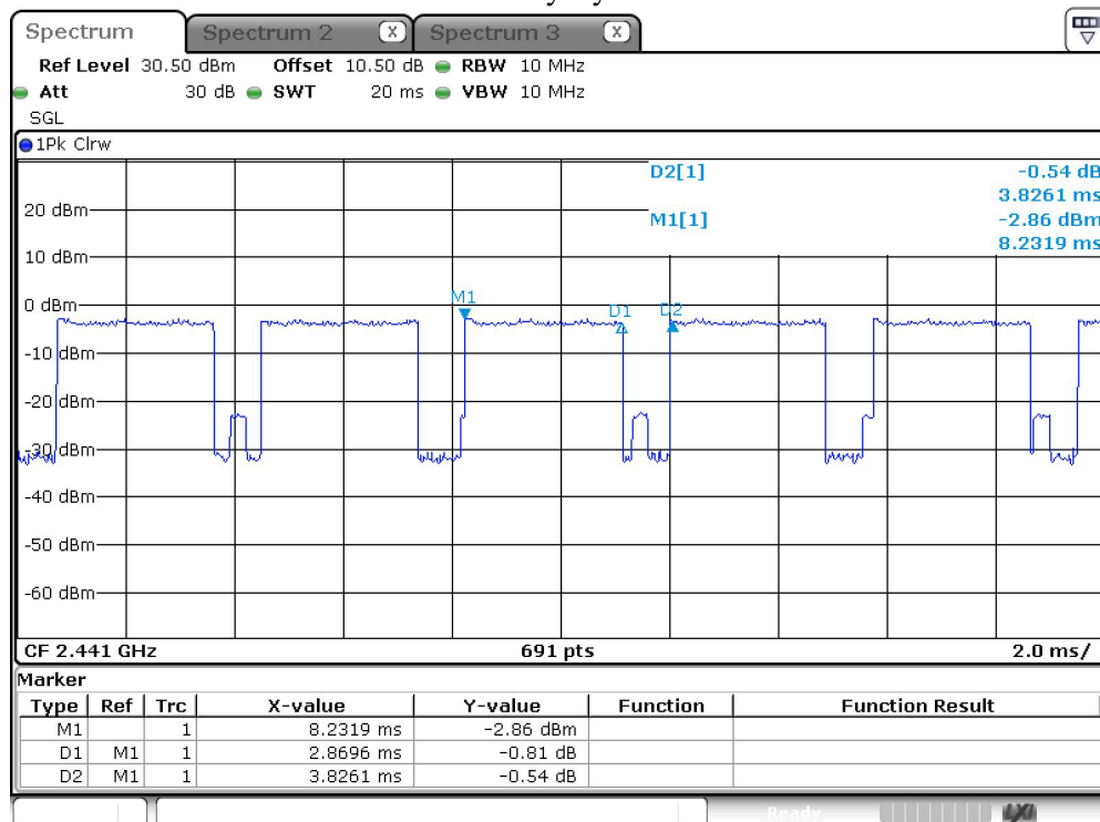
Duty Cycle-3DH5
