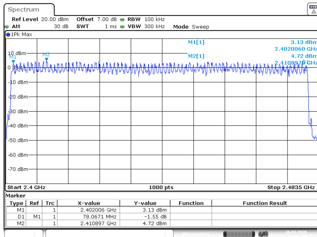
3DH1_Hopping
