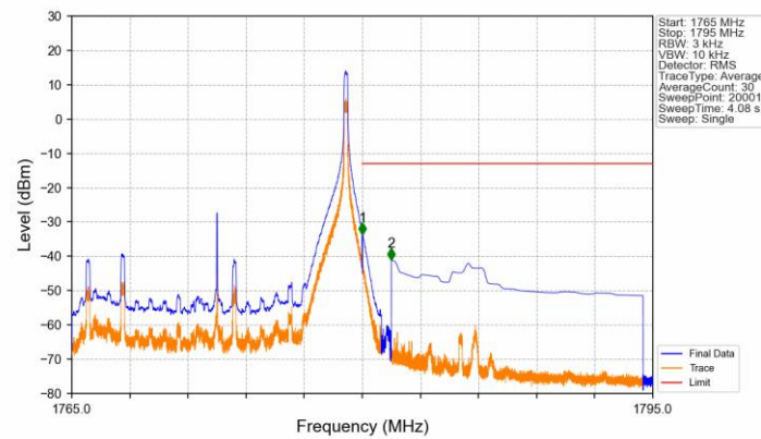
Band66_15MHz_QPSK_HCH_1772.5MHz_RB_1_74_NTNV
