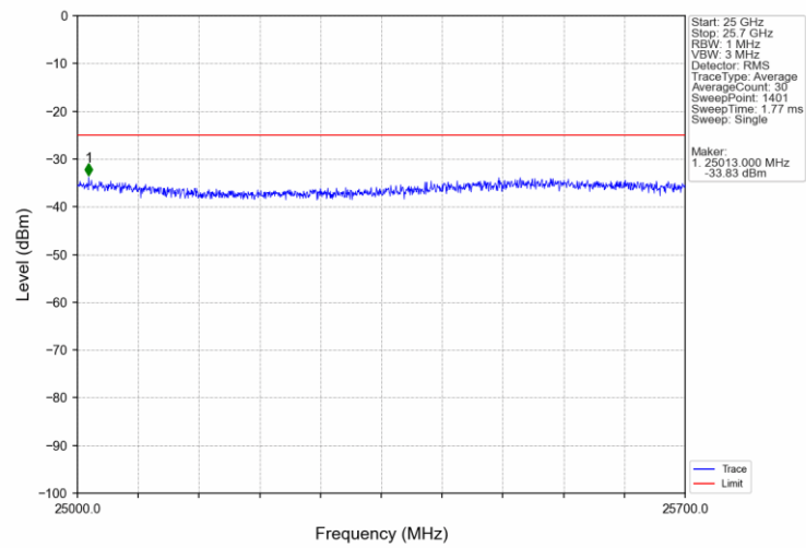
Band7_5MHz_16QAM_MCH_2535MHz_RB_1_0_NTNV
