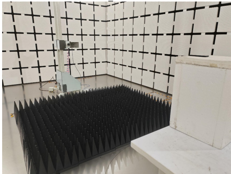
Radiated Above 1GHz
