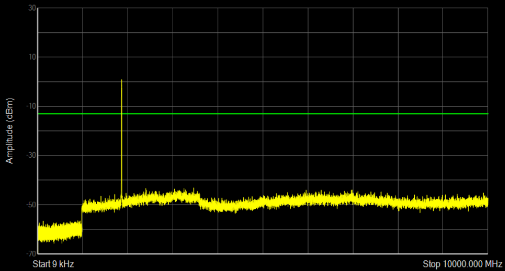
Band25 QPSK BW=10MHz Channel=26365 RB Size=50 Position=#0
