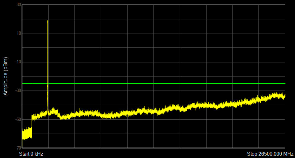
Band41 QAM16 BW=10MHz Channel=40640 RB Size=50 Position=#0
