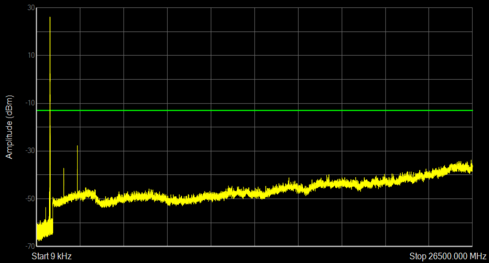
Band5 16QAM BW=5MHz Channel=20525 RB Size=1 Position=#0
