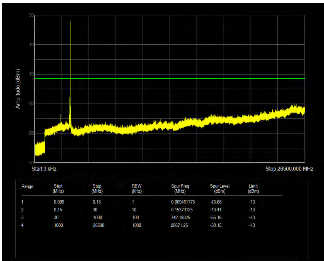
n78 SCS=30kHz CP_QPSK BW=50MHz Channel=635000 RB=133@0
