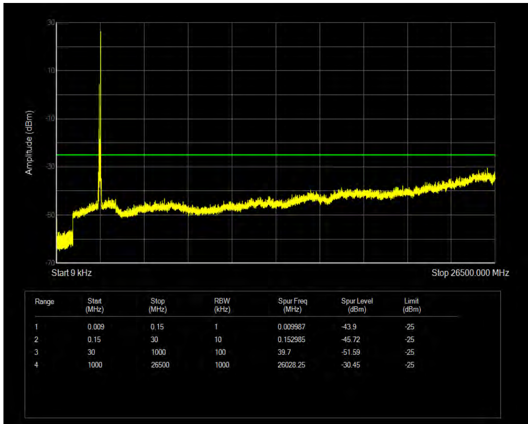
n41 SCS=30kHz CP_QPSK BW=90MHz Channel=528996 RB=245@0
