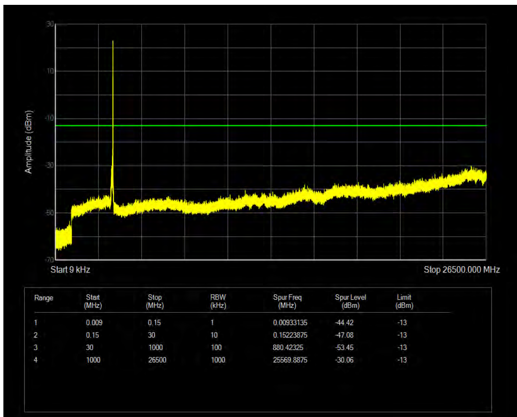
n78 SCS=30kHz CP_QPSK BW=90MHz Channel=633666 RB=245@0
