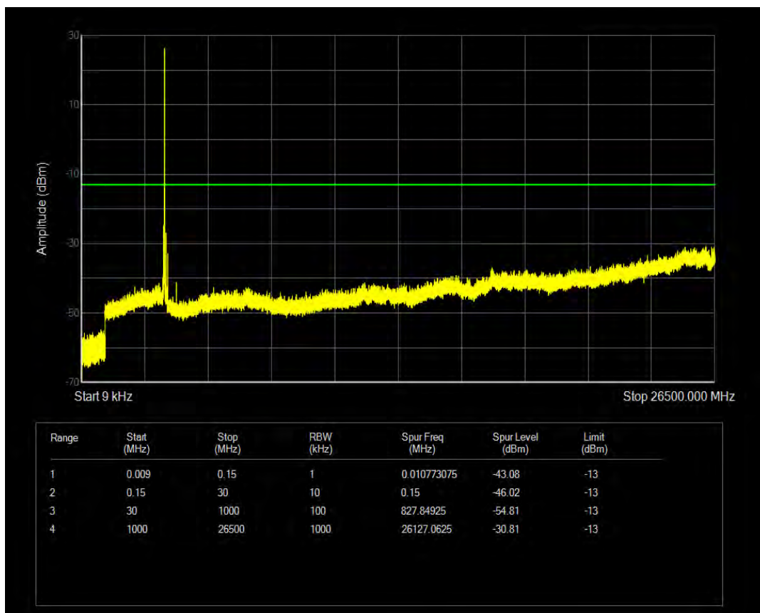
n78 SCS=30kHz CP_QPSK BW=40MHz Channel=635333 RB=106@0
