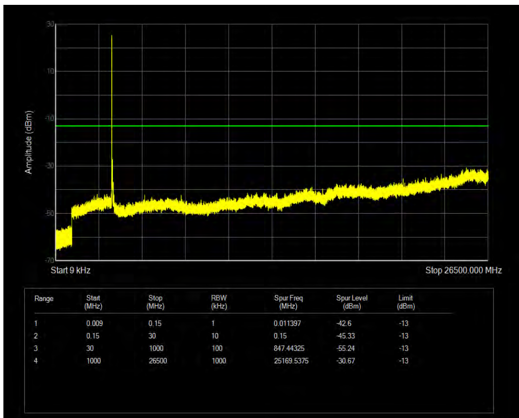
n78 SCS=30kHz CP_QPSK BW=50MHz Channel=631667 RB=1@132
