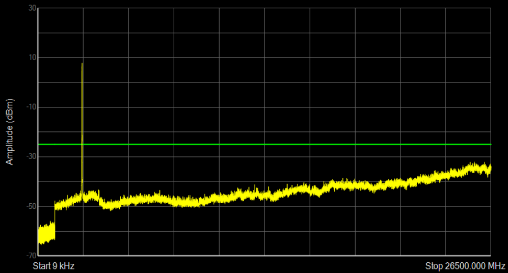
Band41 QPSK BW=15MHz Channel=40620 RB Size=75 Position=#0
