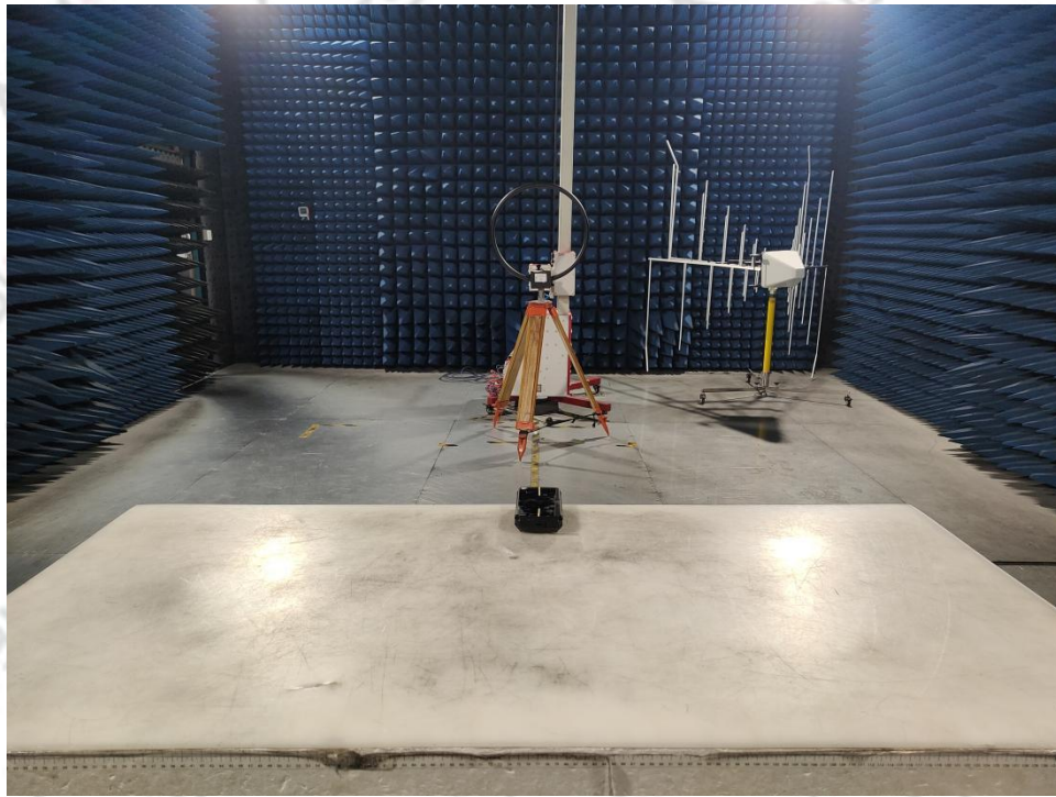
Below 1GHz for NFC
