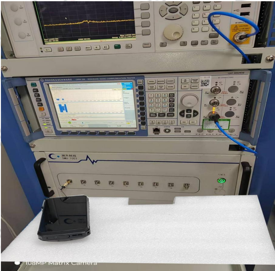
Conducted test photos for GSM/WCDMA/LTE
