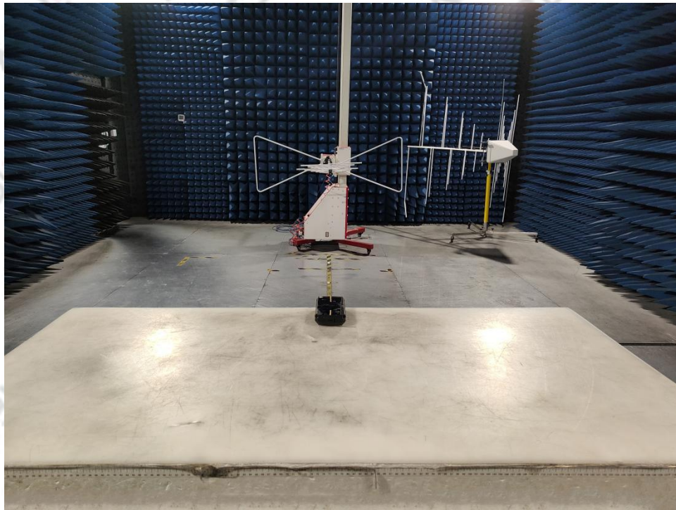
Above 1GHz for GSM/WCDMA/LTE/WIFI BT
