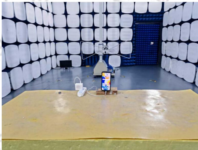
Radiated spurious emission test photos
