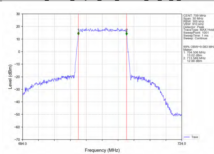
Band17_10MHz_16QAM_LCH_709MHz_RB_50_0_NTNV
