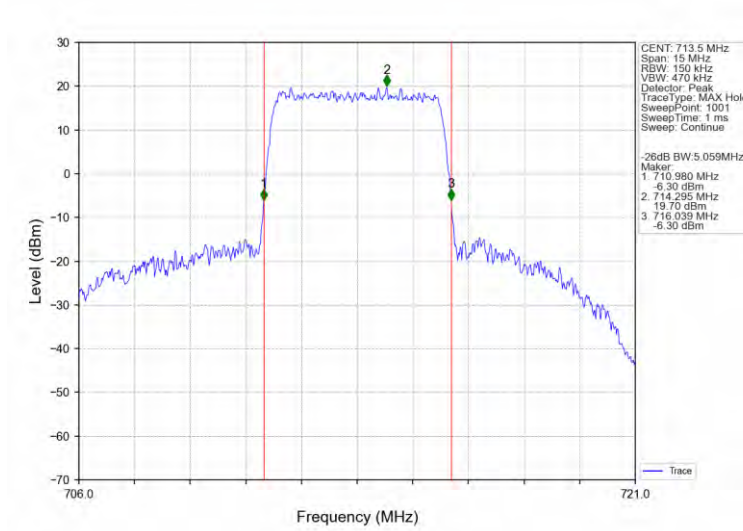
Band17_5MHz_QPSK_HCH_713.5MHz_RB_25_0_NTNV
