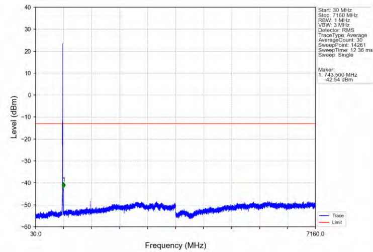
Band17_5MHz_16QAM_HCH_713.5MHz_RB_1_0_NTNV
