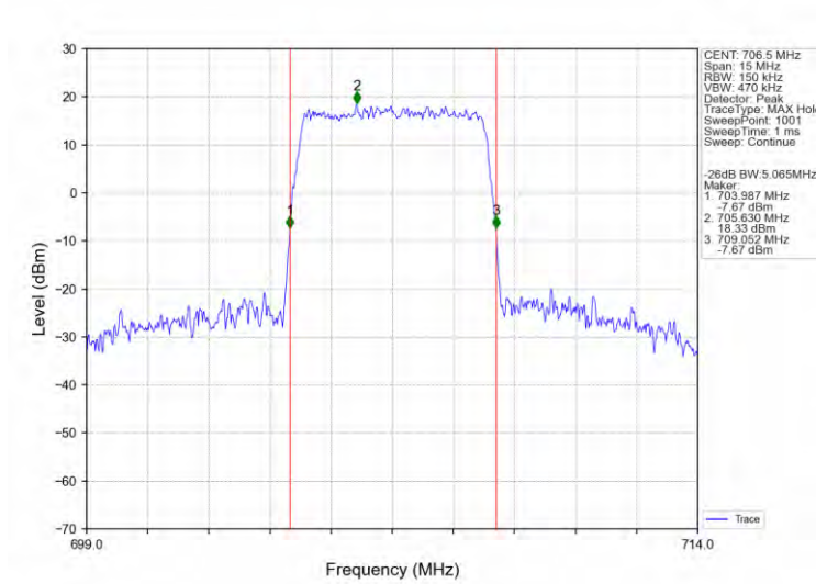
Band17_5MHz_16QAM_LCH_706.5MHz_RB_25_0_NTNV
