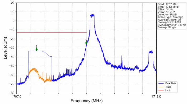
Band66_3MHz_QPSK_LCH_1711.5MHz_RB_1_0_NTNV
