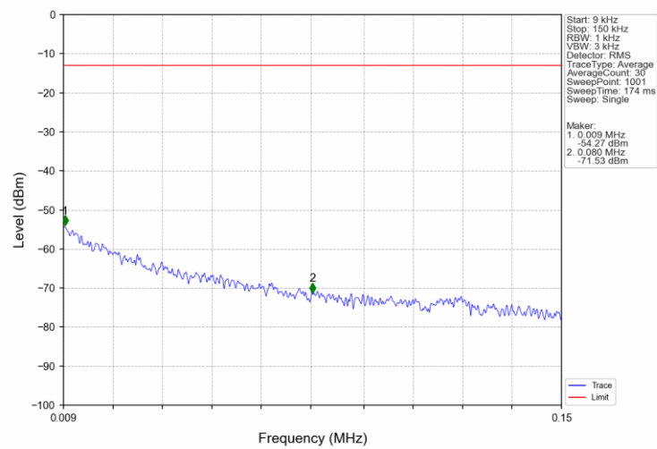
Band66_5MHz_QPSK_LCH_1712.5MHz_RB_1_0_NTNV
