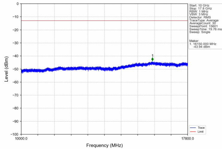
Band66_3MHz_16QAM_LCH_1711.5MHz_RB_15_0_NTNV
