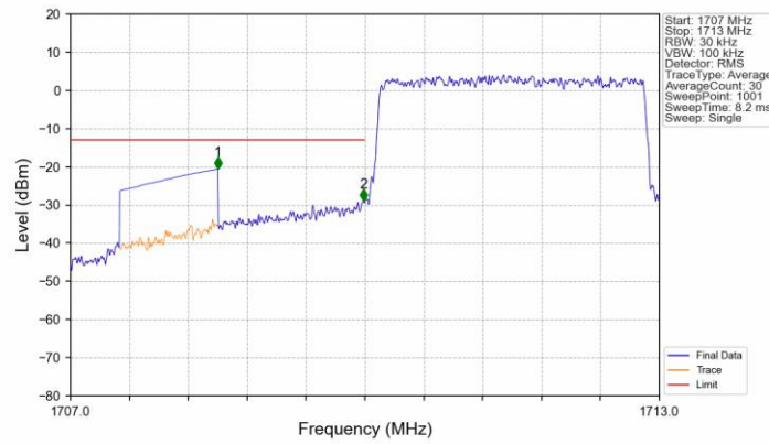
Band66_3MHz_16QAM_LCH_1711.5MHz_RB_15_0_NTNV
