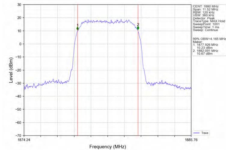
Band2_RMC_MCH_1880MHz_12.2kbps_RMC_NTNV
