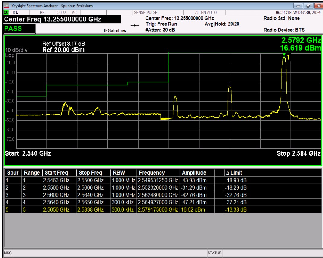
Band41(2565-2645) 16QAM BW=15MHz Channel=40415 RB Size=75 Position=#0
