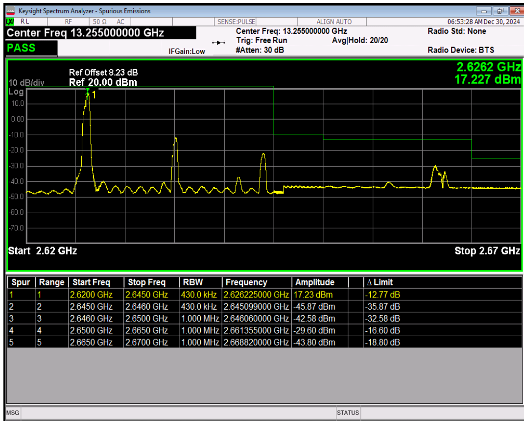
Band41(2565-2645) QPSK BW=20MHz Channel=41040 RB Size=1 Position=#Max
