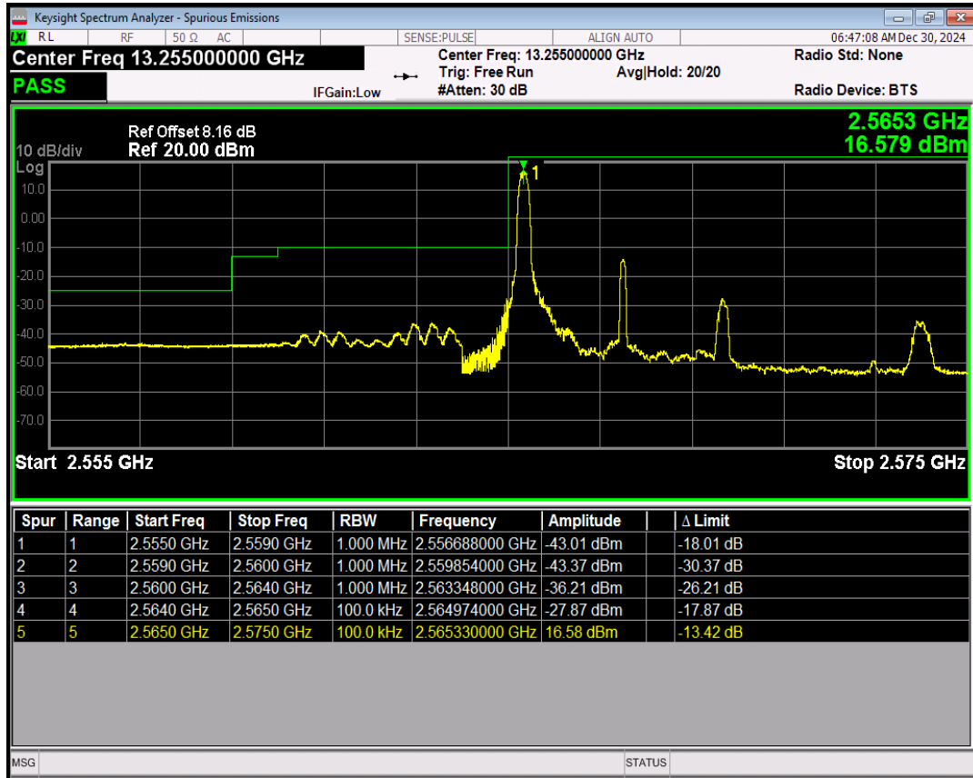
Band41(2565-2645) QPSK BW=5MHz Channel=40365 RB Size=1 Position=#Max
