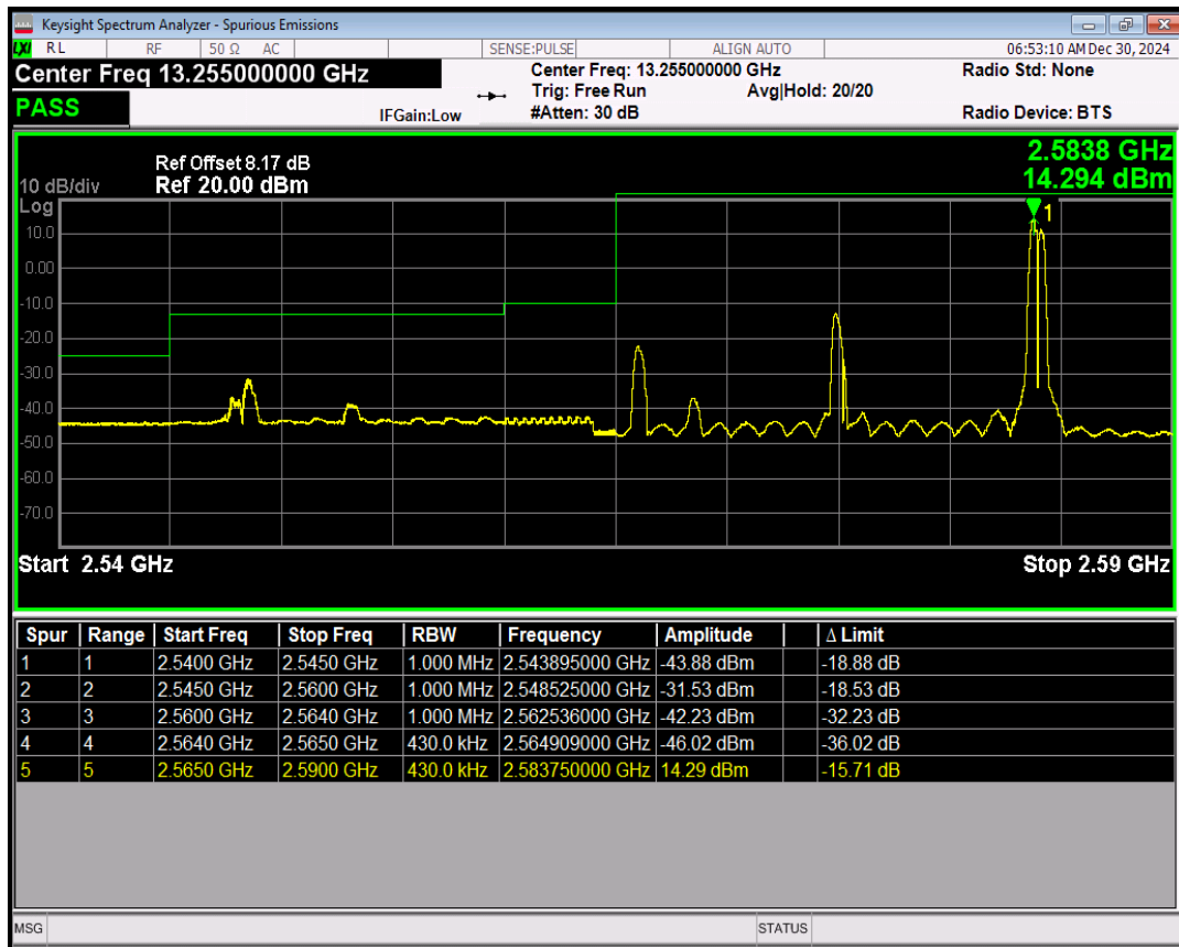
Band41(2565-2645) 16QAM BW=20MHz Channel=40440 RB Size=100 Position=#0
