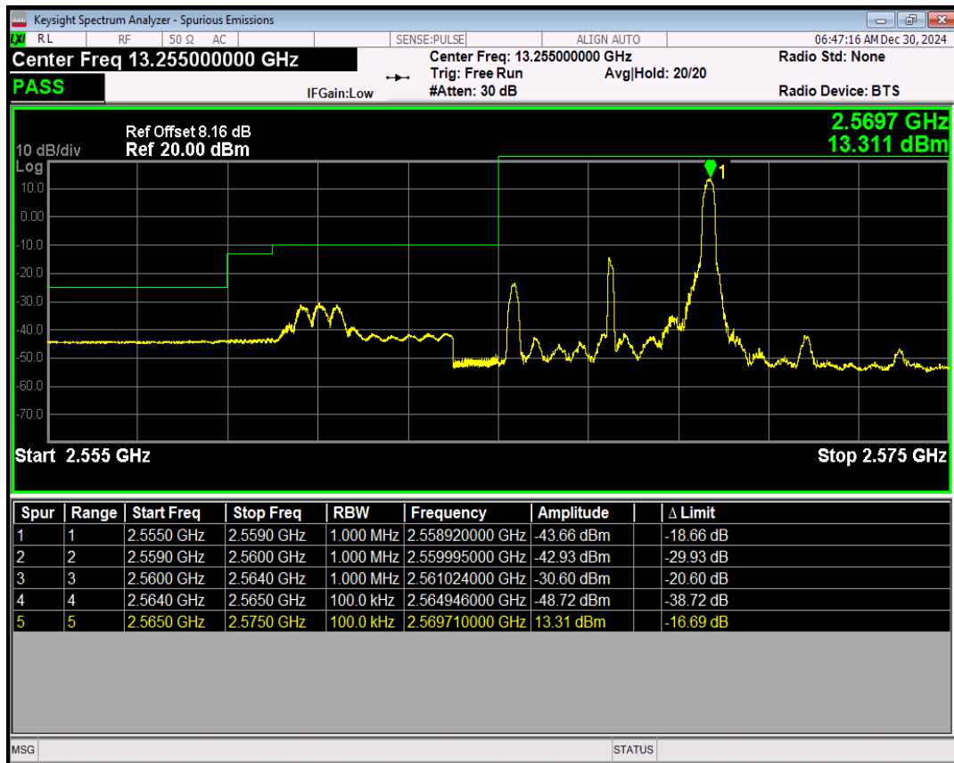
Band41(2565-2645) QPSK BW=5MHz Channel=40365 RB Size=25 Position=#0
