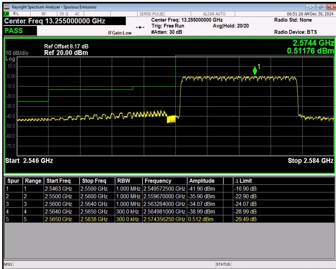
Band41(2565-2645) QPSK BW=15MHz Channel=41065 RB Size=1 Position=#0
