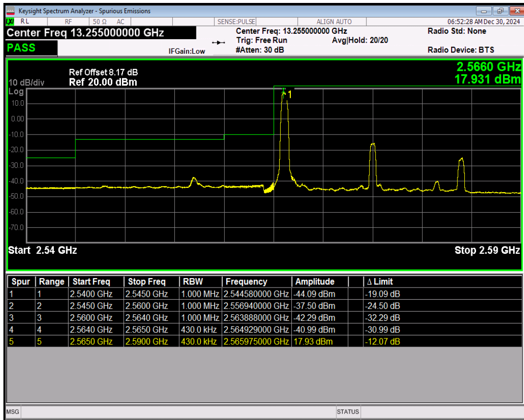
Band41(2565-2645) QPSK BW=20MHz Channel=40440 RB Size=1 Position=#Max
