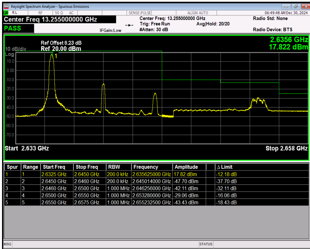
Band41(2565-2645) QPSK BW=10MHz Channel=41090 RB Size=1 Position=#Max
