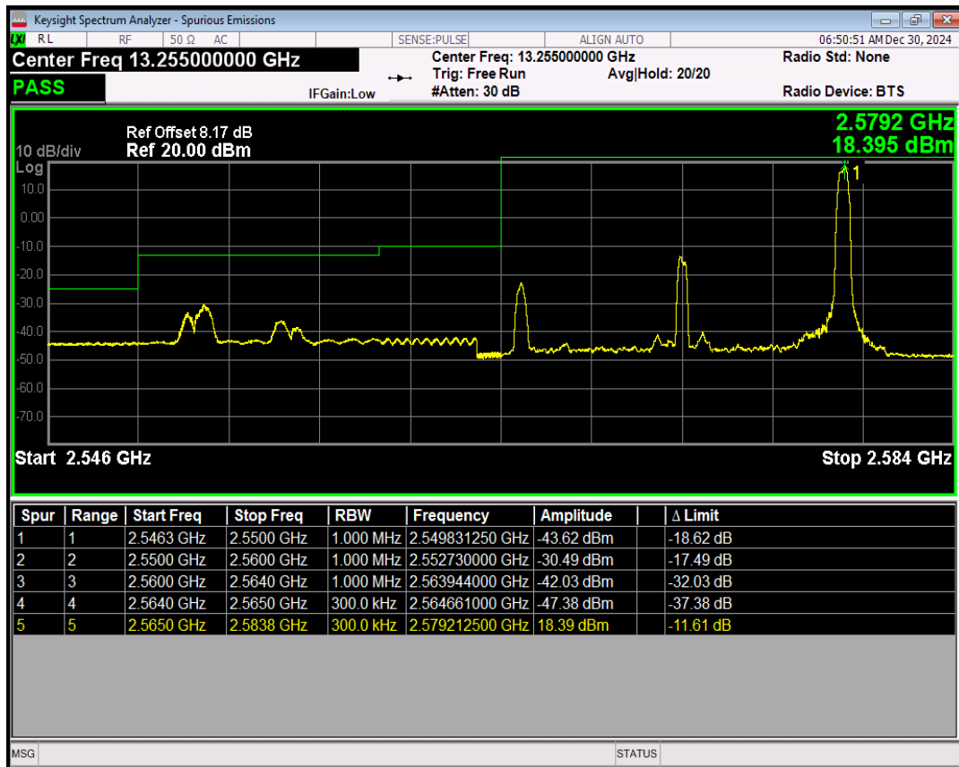
Band41(2565-2645) QPSK BW=15MHz Channel=40415 RB Size=75 Position=#0
