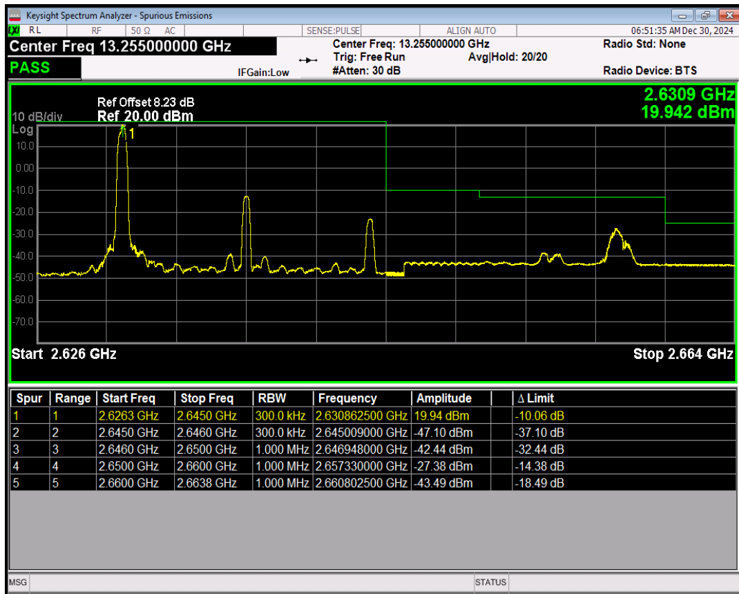
Band41(2565-2645) QPSK BW=15MHz Channel=41065 RB Size=1 Position=#Max
