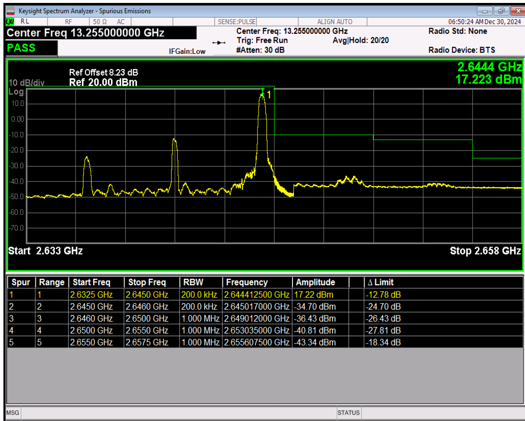
Band41(2565-2645) 16QAM BW=10MHz Channel=41090 RB Size=50 Position=#0
