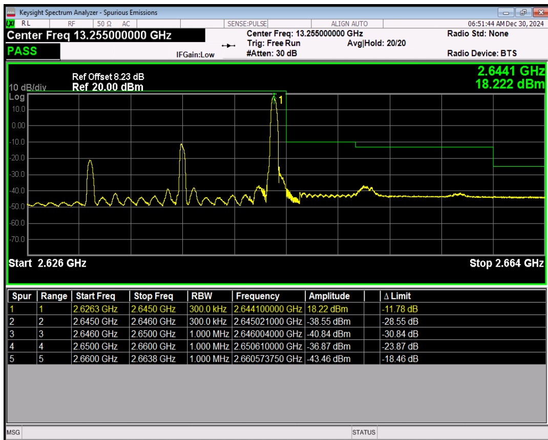
Band41(2565-2645) QPSK BW=15MHz Channel=41065 RB Size=75 Position=#0
