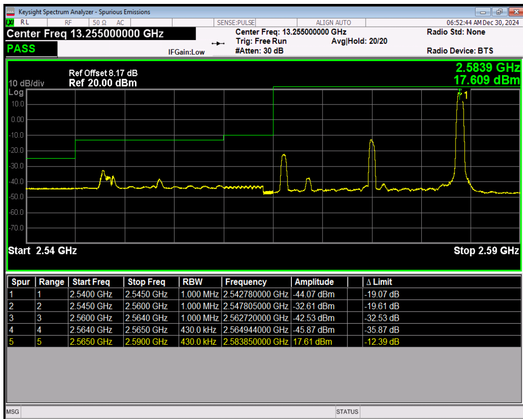
Band41(2565-2645) QPSK BW=20MHz Channel=40440 RB Size=100 Position=#0
