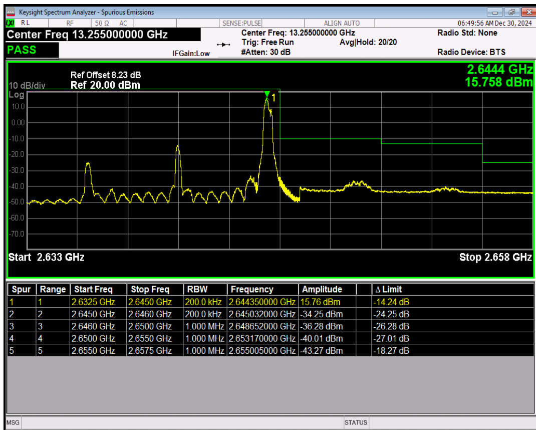
Band41(2565-2645) QPSK BW=10MHz Channel=41090 RB Size=50 Position=#0
