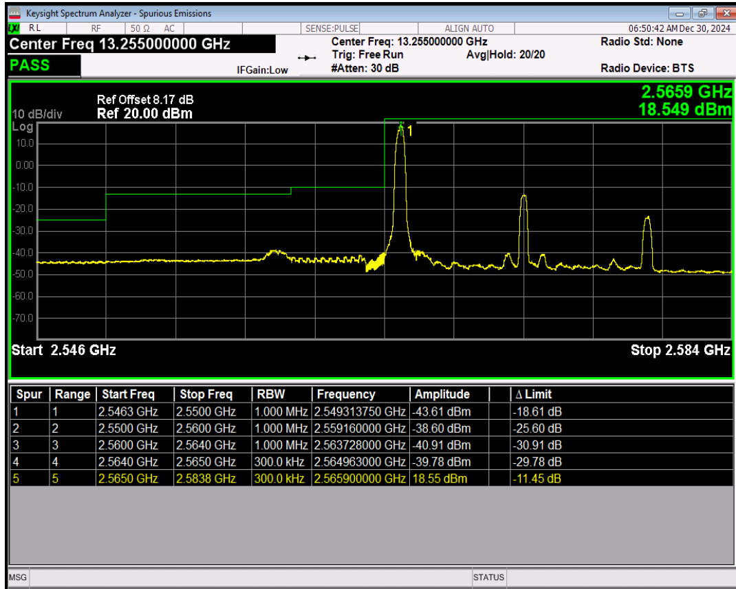
Band41(2565-2645) QPSK BW=15MHz Channel=40415 RB Size=1 Position=#Max
