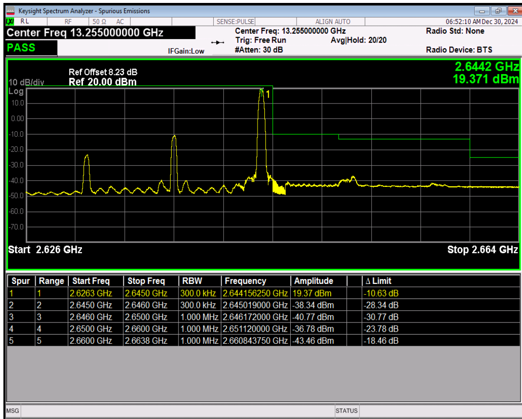
Band41(2565-2645) 16QAM BW=15MHz Channel=41065 RB Size=75 Position=#0
