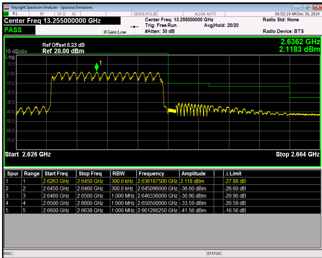
Band41(2565-2645) QPSK BW=20MHz Channel=40440 RB Size=1 Position=#0
