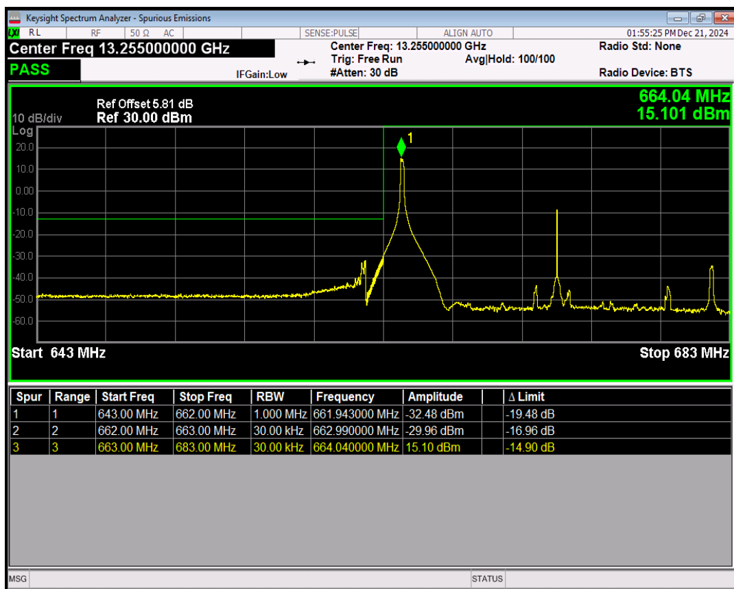
Band71 16QAM BW=20MHz Channel=133222 RB Size=1 Position=#Max
