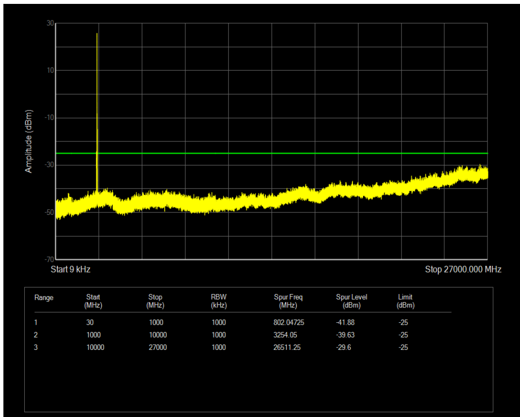
Band41(2565-2645) 16QAM BW=15MHz Channel=40740 RB Size=75 Position=#0
