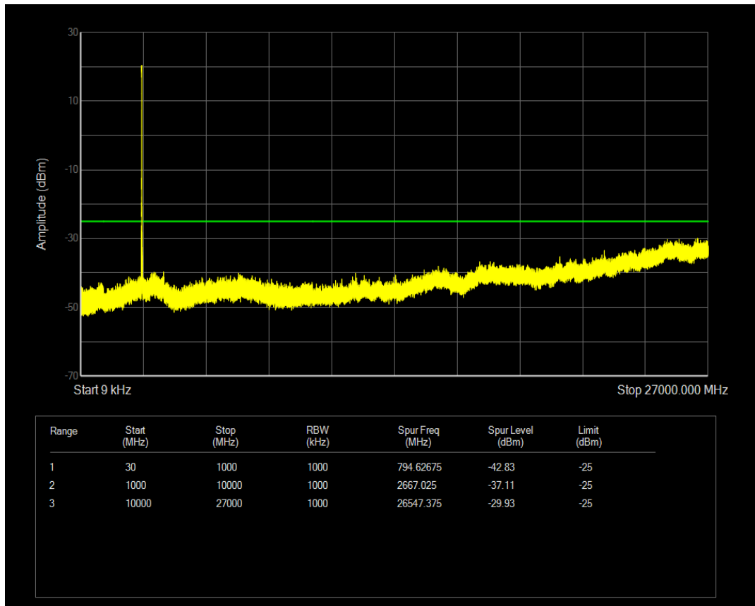
Band41(2565-2645) QPSK BW=10MHz Channel=40390 RB Size=1 Position=#0
