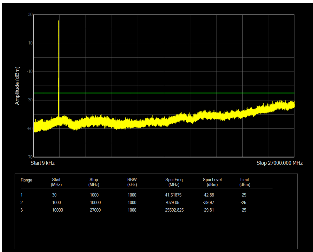
Band41(2565-2645) 16QAM BW=5MHz Channel=40740 RB Size=25 Position=#0
