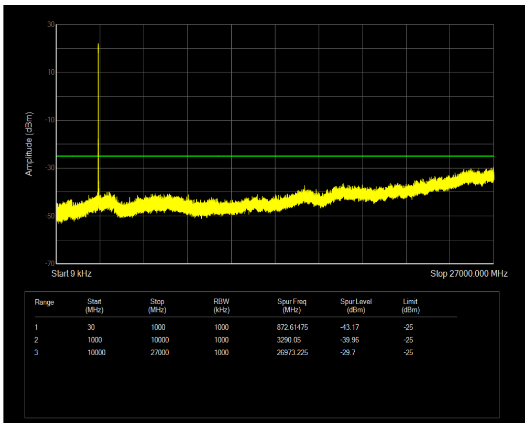
Band41(2565-2645) 16QAM BW=5MHz Channel=40740 RB Size=1 Position=#0
