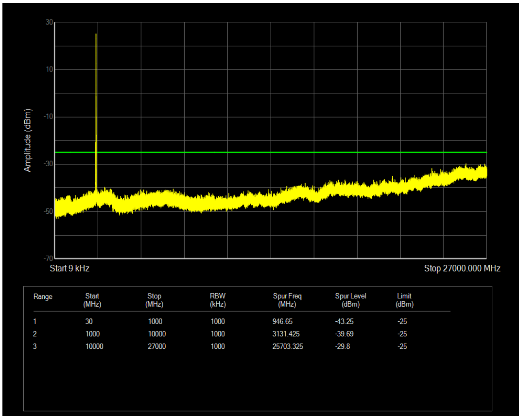
Band41(2565-2645) QPSK BW=15MHz Channel=40740 RB Size=75 Position=#0
