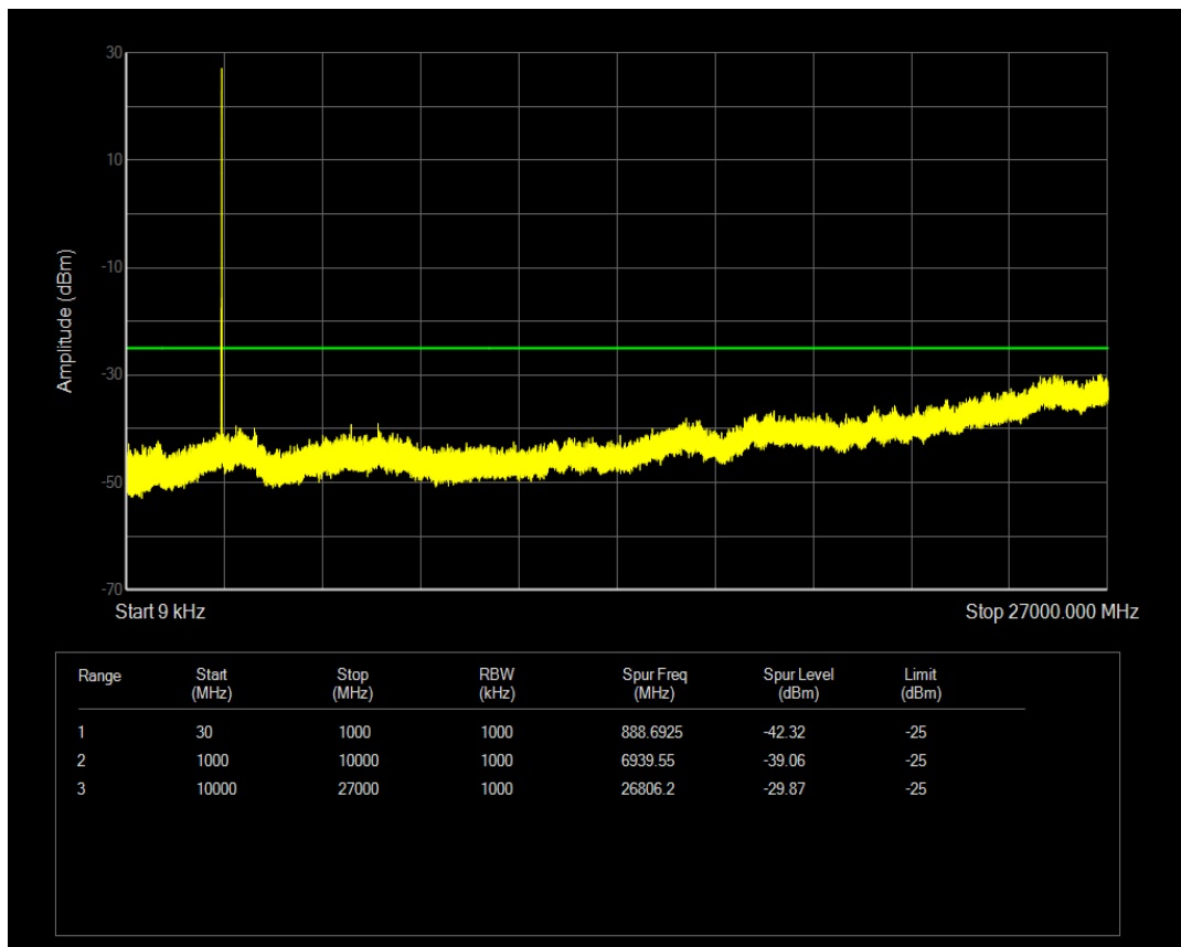
Band41(2565-2645) 16QAM BW=5MHz Channel=41115 RB Size=25 Position=#0
