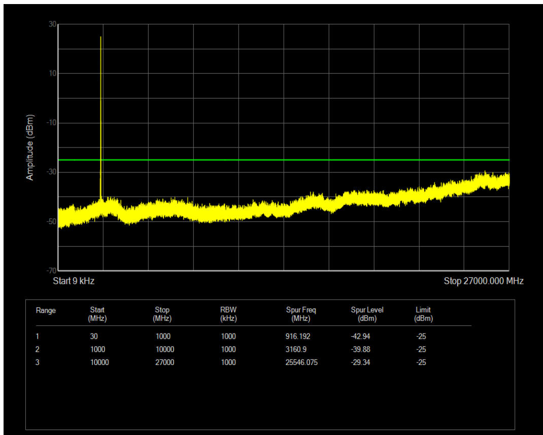
Band41(2565-2645) 16QAM BW=10MHz Channel=40390 RB Size=50 Position=#0
