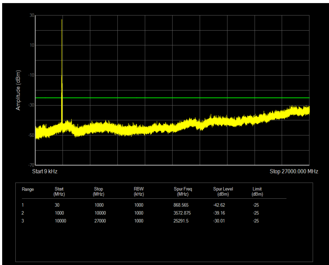
Band41(2565-2645) QPSK BW=20MHz Channel=41040 RB Size=100 Position=#0
