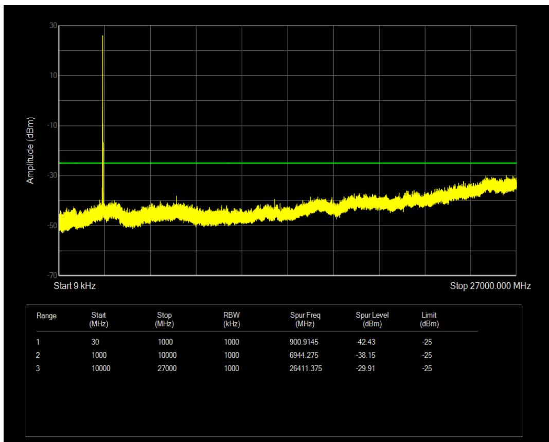
Band41(2565-2645) 16QAM BW=20MHz Channel=40740 RB Size=100 Position=#0
