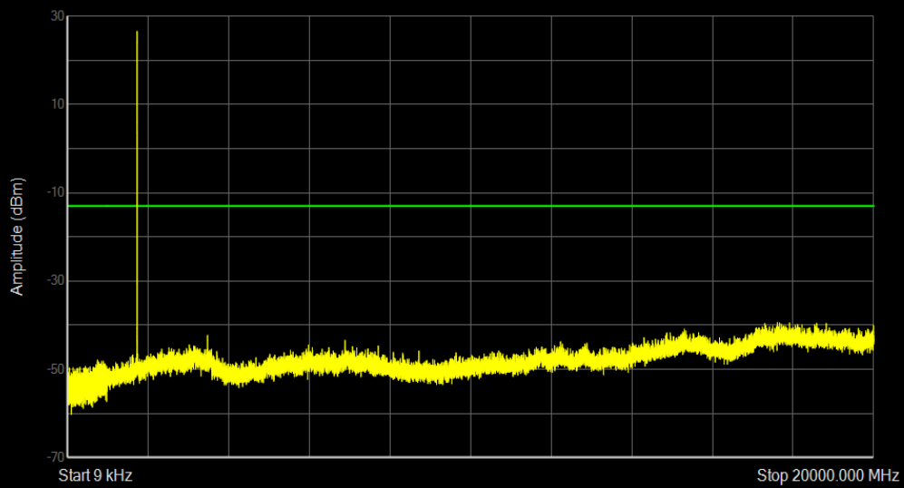
Band66 16QAM BW=1.4MHz Channel=132322 RB Size=1 Position=#0
