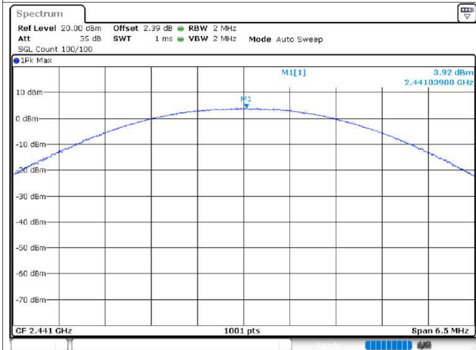
Power NVNT 2-DH5 2441MHz Ant1
