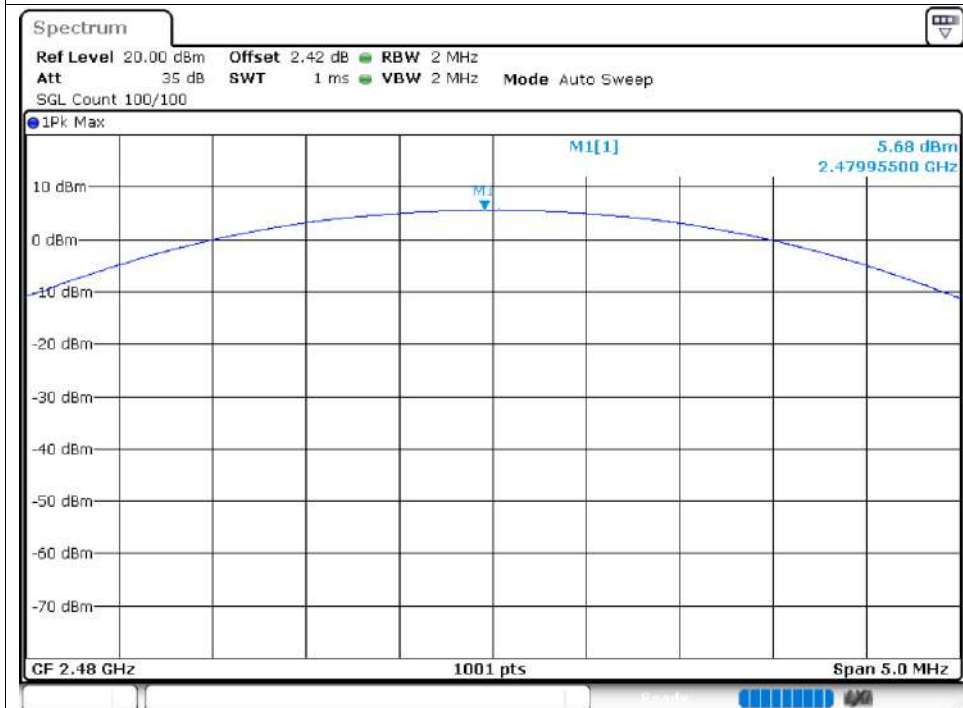
Power NVNT 1-DH5 2480MHz Ant1
