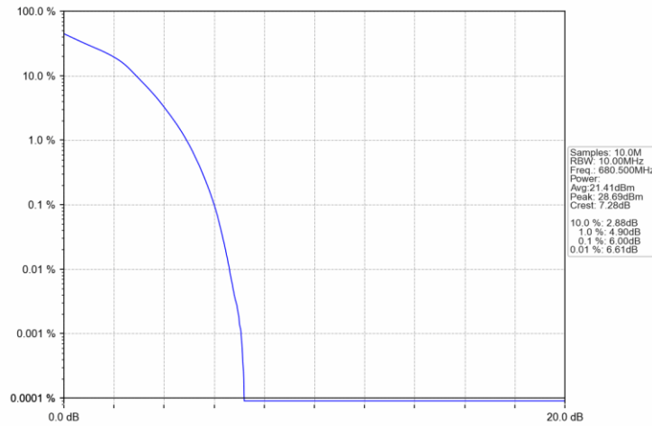
Band71_10MHz_16QAM_MCH_680.5MHz_RB_50_0_NTNV
