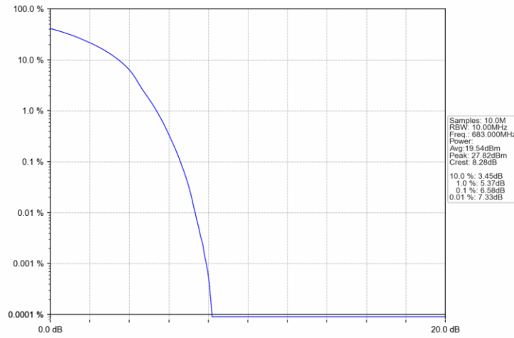
Band71_20MHz_16QAM_MCH_683MHz_RB_100_0_NTNV
