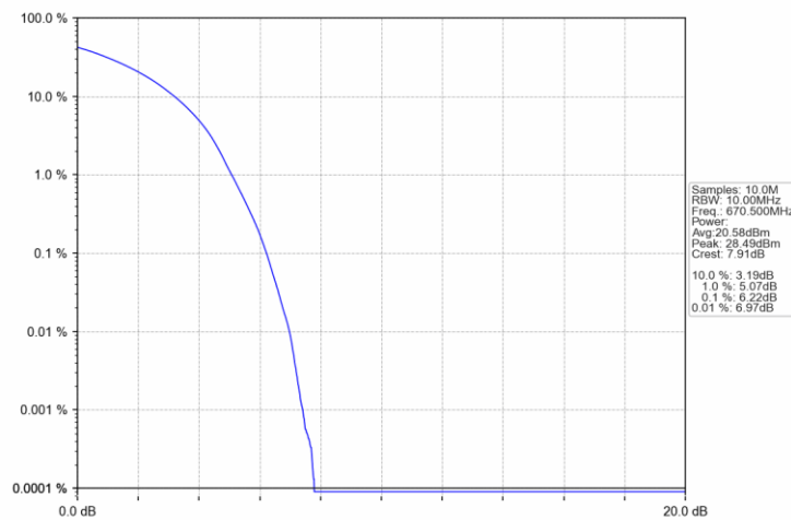
Band71_15MHz_16QAM_LCH_670.5MHz_RB_75_0_NTNV
