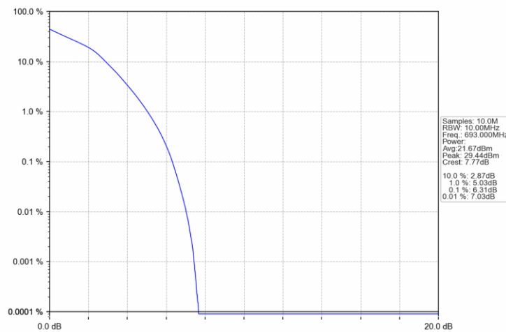
Band71_10MHz_16QAM_HCH_693MHz_RB_50_0_NTNV
