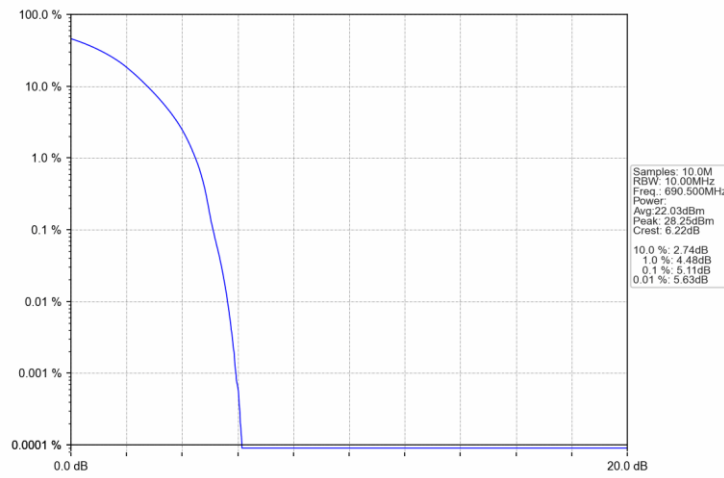
Band71_15MHz_QPSK_HCH_690.5MHz_RB_75_0_NTNV
