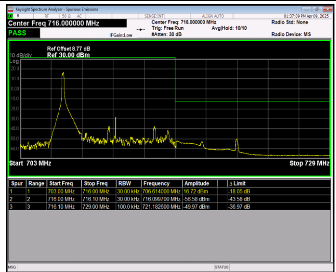
Band12-10MHz-64QAM-23130-50RB#0
