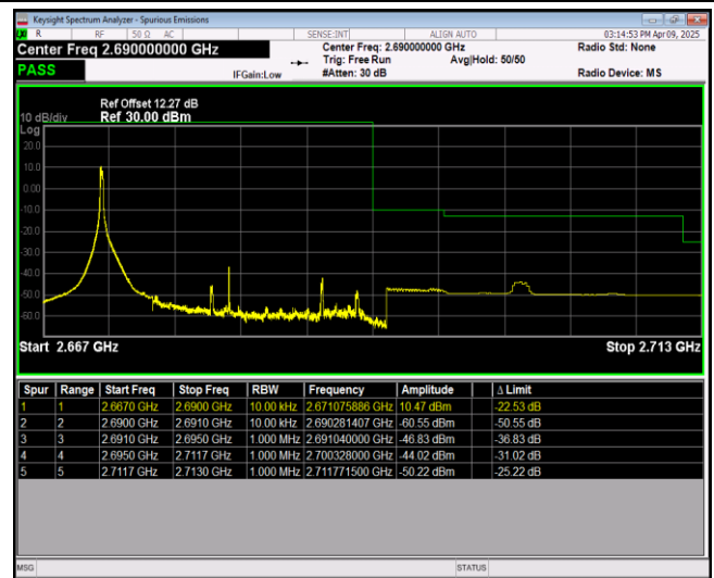
Band41-20MHz-QPSK-41490-100RB#0
