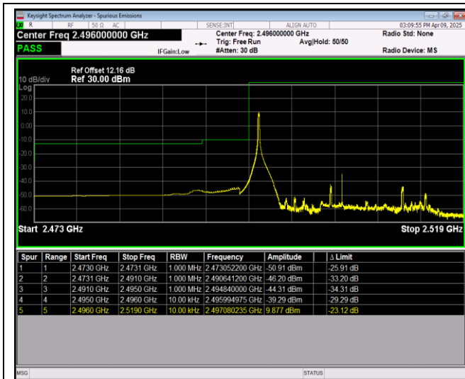
Band41-20MHz-QPSK-39750-100RB#0
