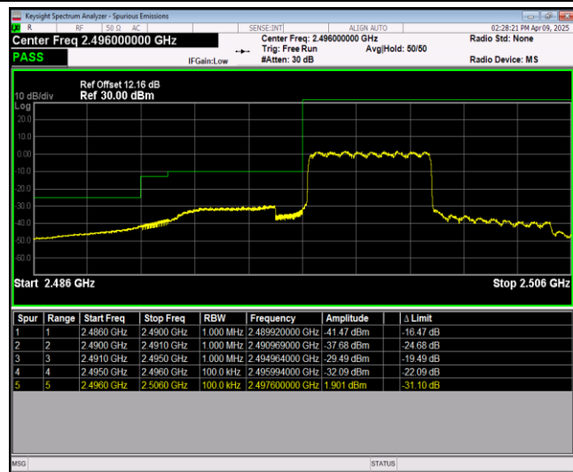
Band41-5MHz-QPSK-41565-1RB#24
