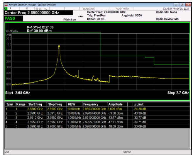
Band41-5MHz-16QAM-41565-25RB#0
