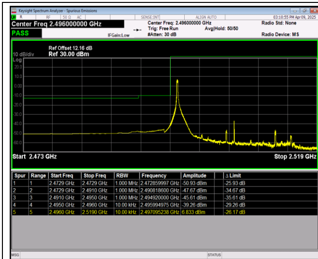
Band41-20MHz-64QAM-39750-100RB#0
