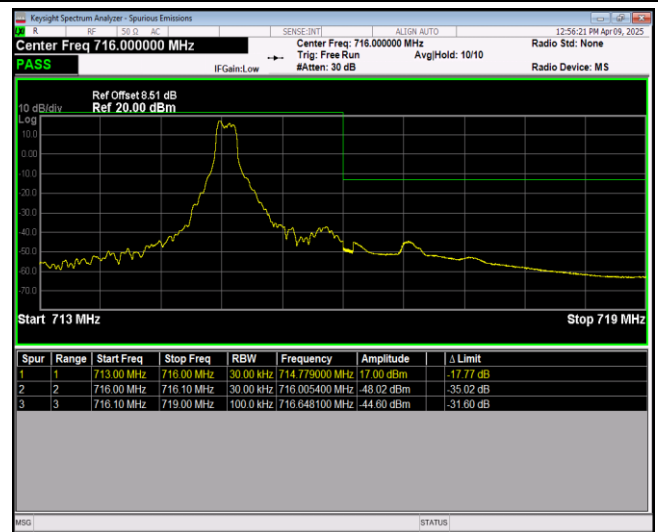
Band12-1.4MHz-64QAM-23173-6RB#0
