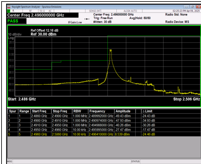
Band41-5MHz-QPSK-39675-25RB#0
