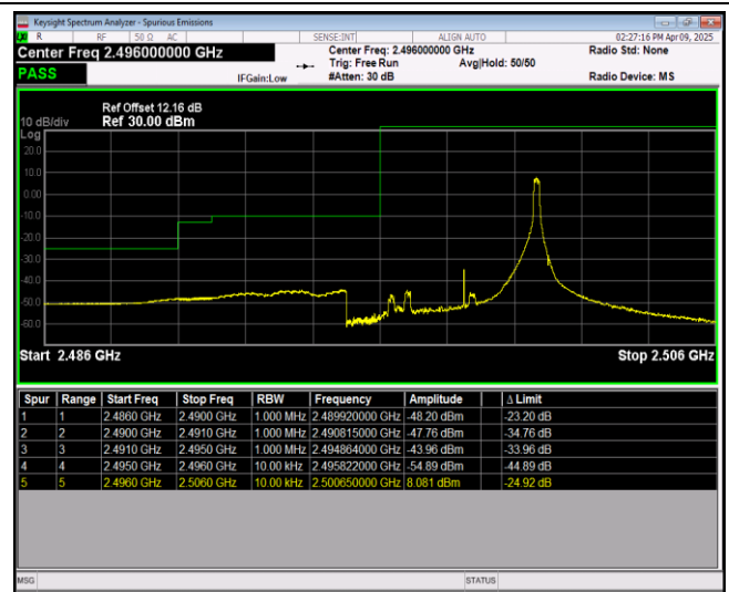
Band41-5MHz-16QAM-41565-1RB#0
