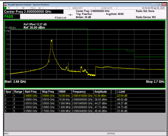
Band41-5MHz-QPSK-41565-25RB#0
