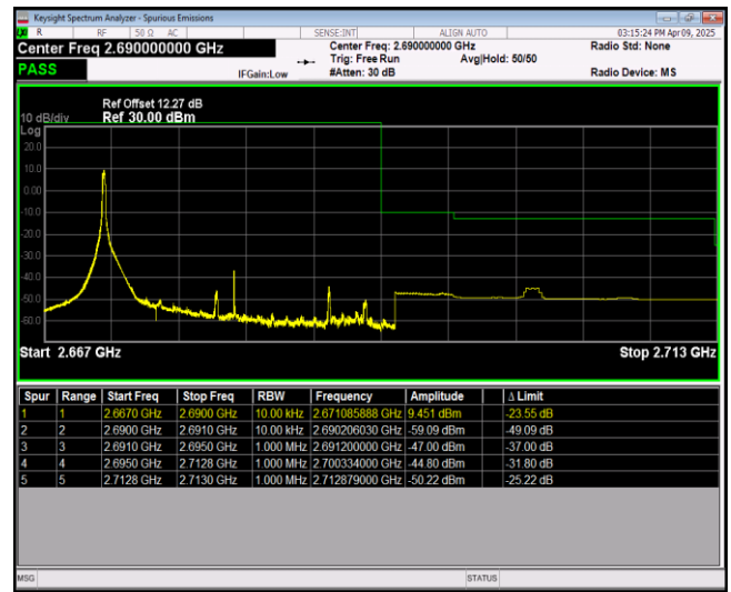
Band41-20MHz-16QAM-41490-100RB#0
