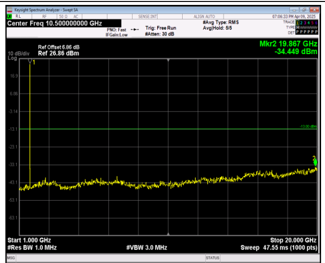
Band66-1.4MHz-QPSK-132322-1RB#0-Range2:1000~20000MHz
