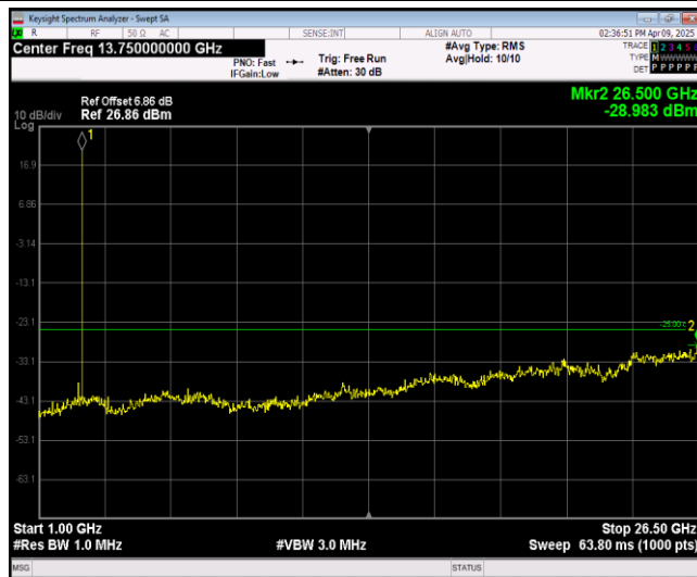
Band41-5MHz-16QAM-39675-1RB#0-Range2:1000~ 26500MHz
