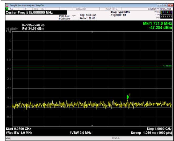
Band66-1.4MHz-QPSK-132322-1RB#0-Range1:30~1000MHz
