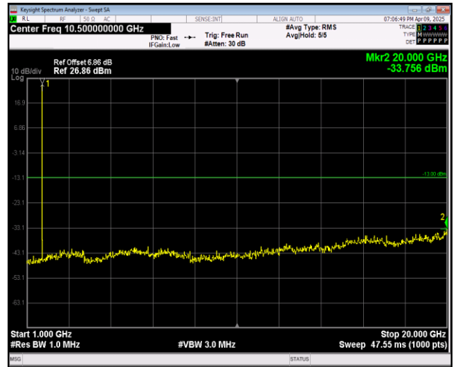
Band66-1.4MHz-16QAM-132322-1RB#0-Range2:1000~20000MHz
