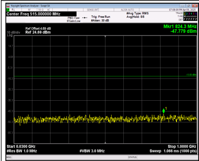
Band66-1.4MHz-QPSK-132665-1RB#0-Range1:30~1000MHz
