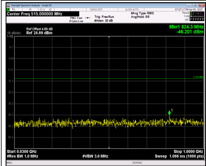
Band66-1.4MHz-QPSK-132665-1RB#0-Range1:30~1000MHz
