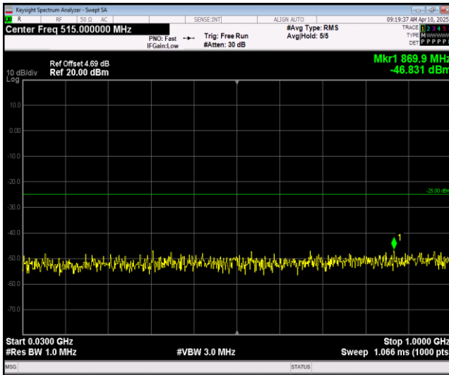
Band41-20MHz-16QAM-39750-1RB#0-Range1:30~1000MHz
