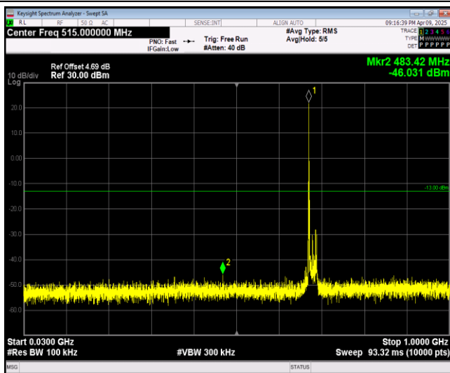
Band71-20MHz-16QAM-133222-1RB#0-Range1:30~ 1000MHz
