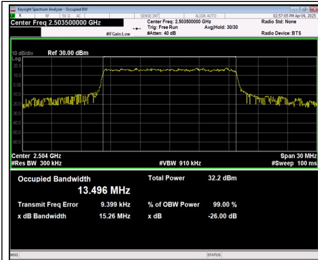
Band41-15MHz-QPSK-41515-75RB#0
