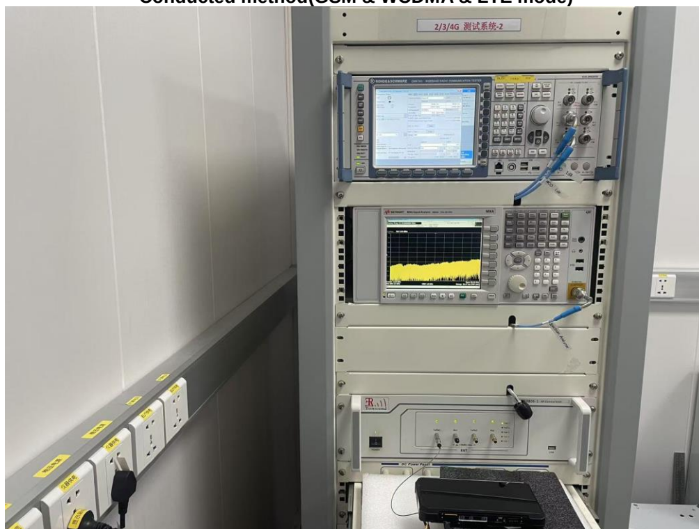
Conducted method(GSM & WCDMA & LTE mode)
