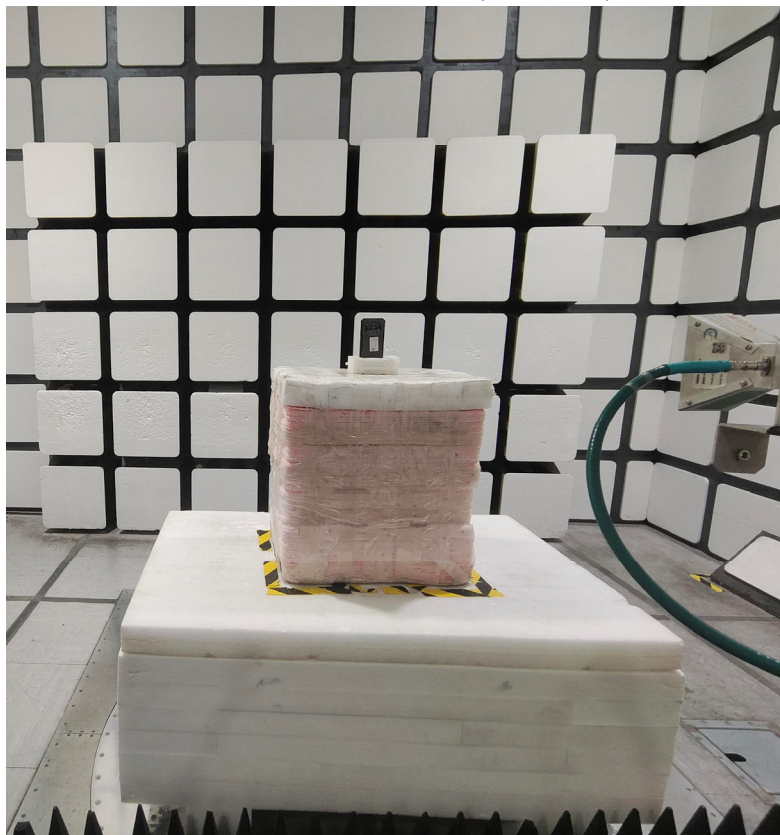
Radiated Emissions View (18-40 GHz)
