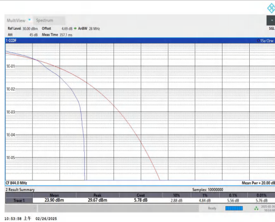
Band5-10MHz-16QAM-20600-1RB#0-PASS
