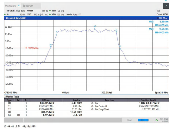
Band5-1.4MHz-QPSK-20525-6RB#0-PASS
