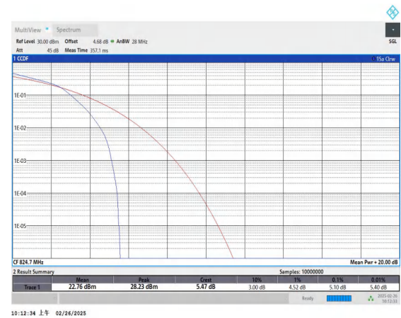
Band5-1.4MHz-16QAM-20407-6RB#0-PASS
