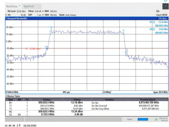
Band5-10MHz-16QAM-20600-50RB#0-PASS
