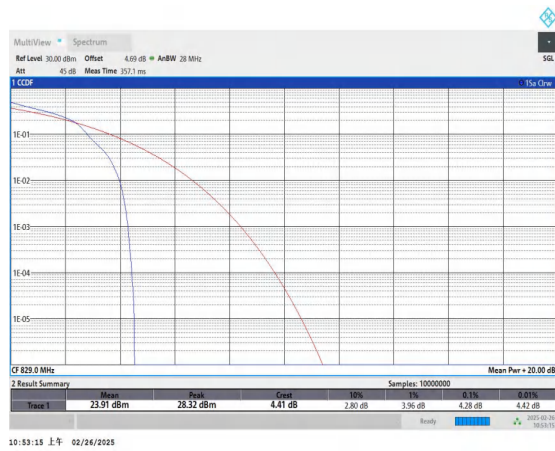
Band5-10MHz-16QAM-20450-1RB#0-PASS
