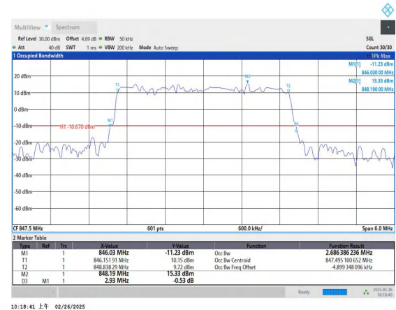
Band5-3MHz-16QAM-20635-15RB#0-PASS
