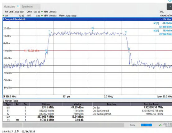
Band5-10MHz-16QAM-20525-50RB#0-PASS
