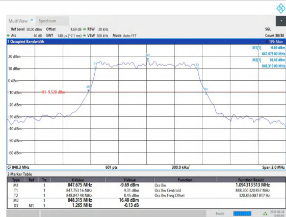
Band5-1.4MHz-16QAM-20643-6RB#0-PASS
