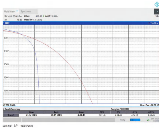
Band5-10MHz-16QAM-20525-1RB#0-PASS
