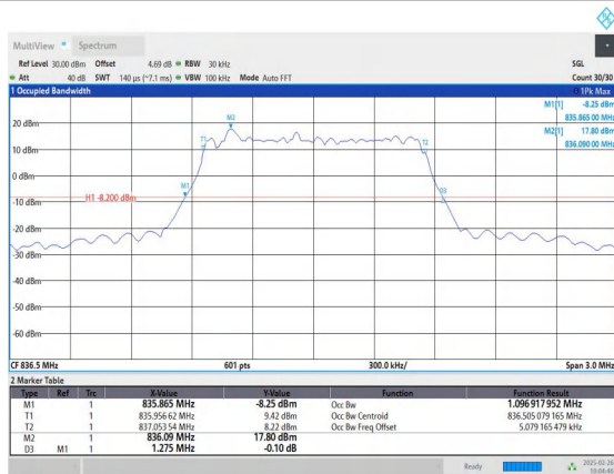
Band5-1.4MHz-16QAM-20525-6RB#0-PASS
