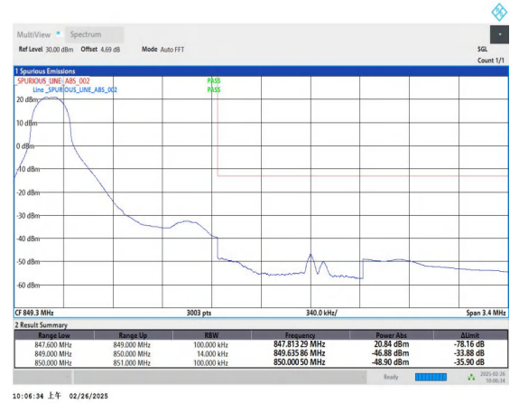
Band5_1.4MHz_16QAM_20643_1RB#0
