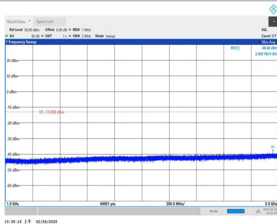
Band5_5MHz_QPSK_20525_1RB#0_1000~3000_1000~3000
