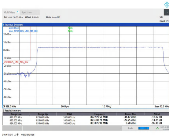
Band5_10MHz_16QAM_20450_50RB#0
