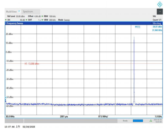
Band5_1.4MHz_16QAM_20407_1RB#0_30~1000_30~1000
