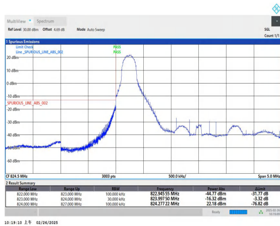
Band5_3MHz_16QAM_20415_1RB#0
