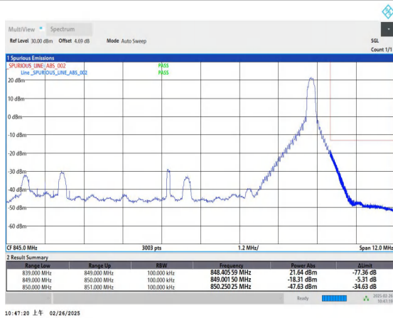
Band5_10MHz_16QAM_20600_1RB#49
