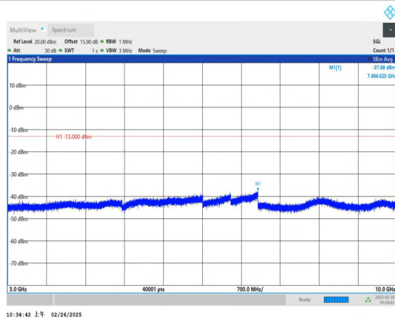
Band5_5MHz_QPSK_20425_1RB#0_3000~10000_3000~10000
