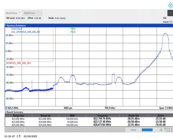
Band5_5MHz_QPSK_20425_1RB#24
