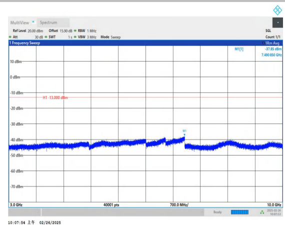
Band5_1.4MHz_16QAM_20407_1RB#0_3000~10000_3000~10000
