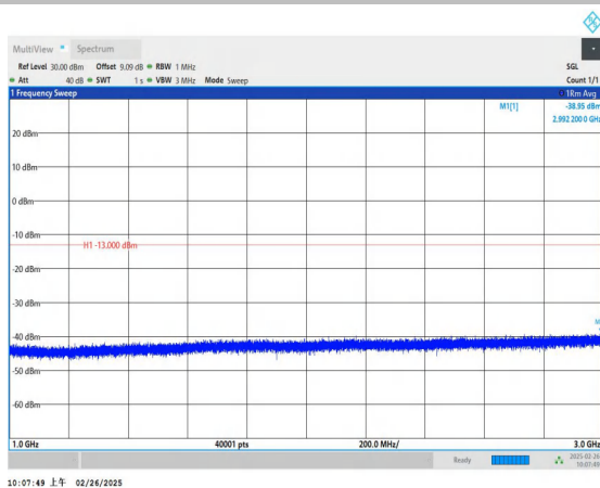
Band5_1.4MHz_16QAM_20407_1RB#0_1000~3000_1000~3000
