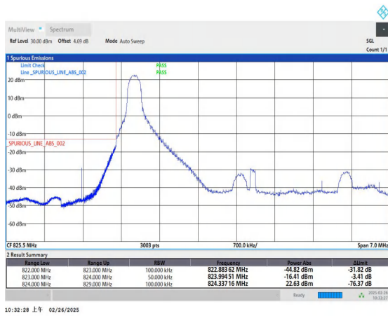
Band5_5MHz_QPSK_20425_1RB#0
