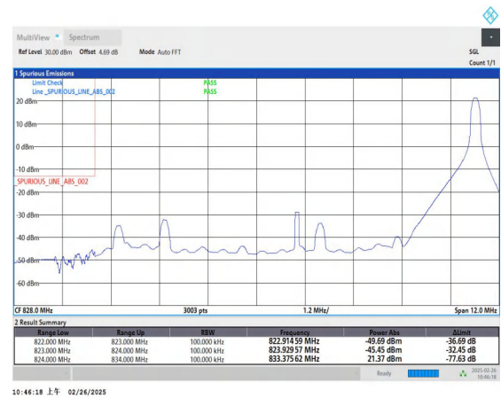
Band5_10MHz_16QAM_20450_1RB#49
