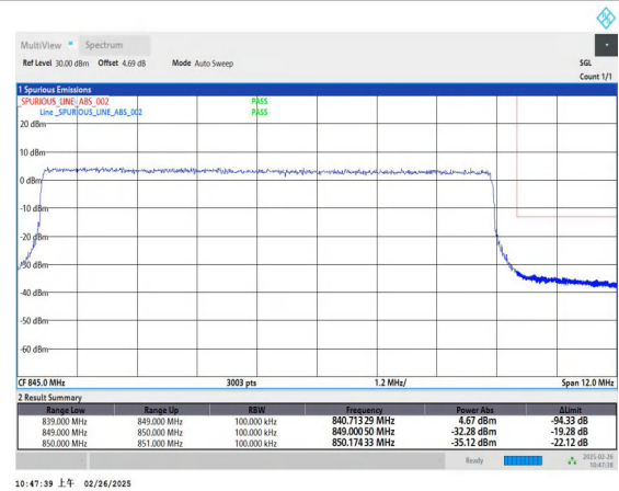
Band5_10MHz_16QAM_20600_50RB#0
