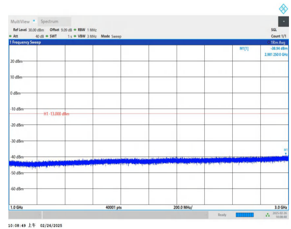
Band5_1.4MHz_QPSK_20643_1RB#0_1000~3000_1000~3000
