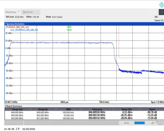
Band5_5MHz_QPSK_20625_25RB#0
