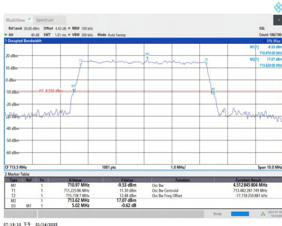
Band17-5MHz-QPSK-23825-25RB#0-PASS
