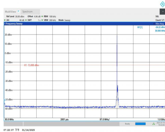
Band17_5MHz_QPSK_23790_1RB#0_30~1000_30~1000
