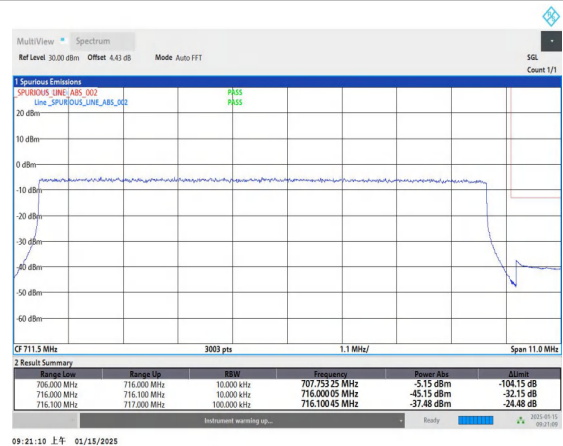
Band17_10MHz_16QAM_23800_50RB#0
