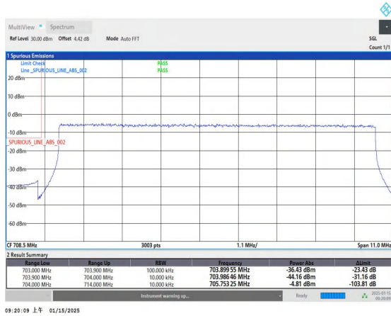
Band17_10MHz_16QAM_23780_50RB#0
