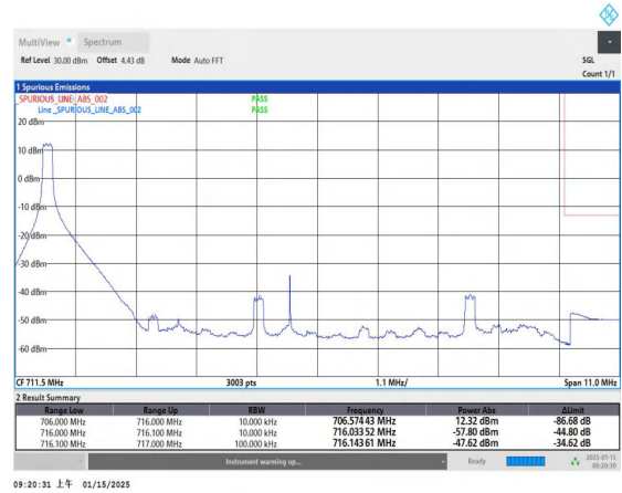
Band17_10MHz_16QAM_23800_1RB#0
