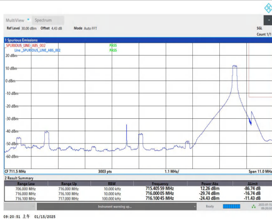
Band17_10MHz_16QAM_23800_1RB#49
