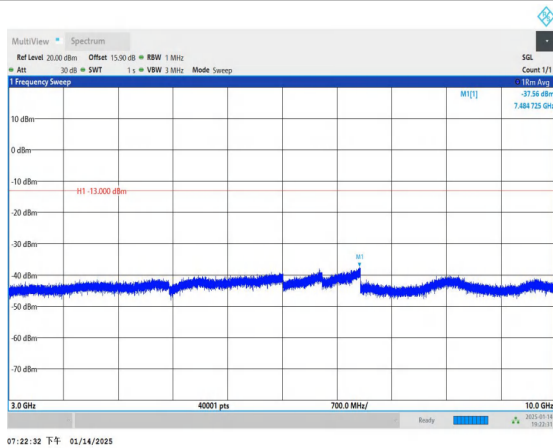
Band17_5MHz_16QAM_23790_1RB#0_3000~10000_3000~10
