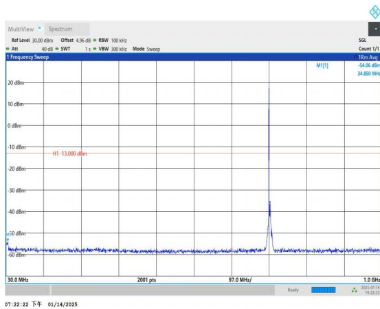
Band17_5MHz_16QAM_23790_1RB#0_30~1000_30~1000
