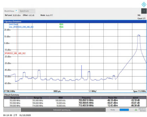
Band17_10MHz_16QAM_23780_1RB#49
