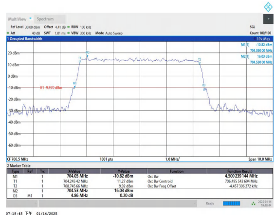
Band17-5MHz-16QAM-23755-25RB#0-PASS
