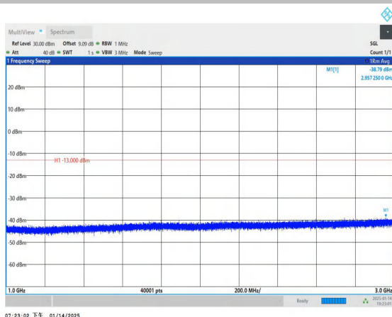
Band17_5MHz_16QAM_23825_1RB#0_1000~3000_1000~300
