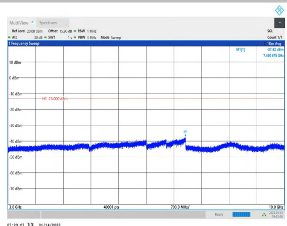
Band17_5MHz_16QAM_23825_1RB#0_3000~10000_3000~10
