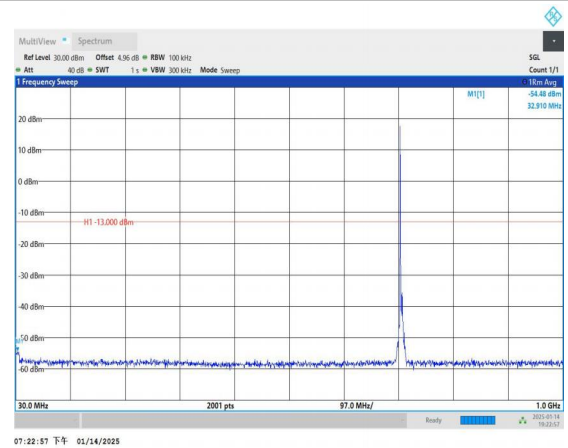
Band17_5MHz_16QAM_23825_1RB#0_30~1000_30~1000
