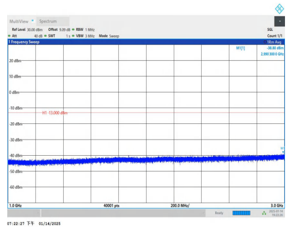
Band17_5MHz_16QAM_23790_1RB#0_1000~3000_1000~300
