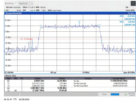
Band41-20MHz-16QAM-41490-100RB#0-PASS
