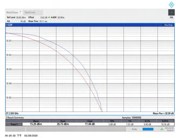
Band41-20MHz-QPSK-40620-100RB#0-PASS
