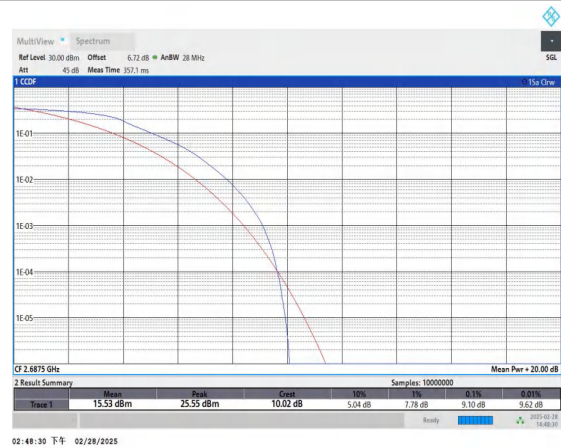
Band41-5MHz-QPSK-41565-25RB#0-PASS
