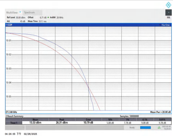
Band41-20MHz-QPSK-41490-100RB#0-PASS
