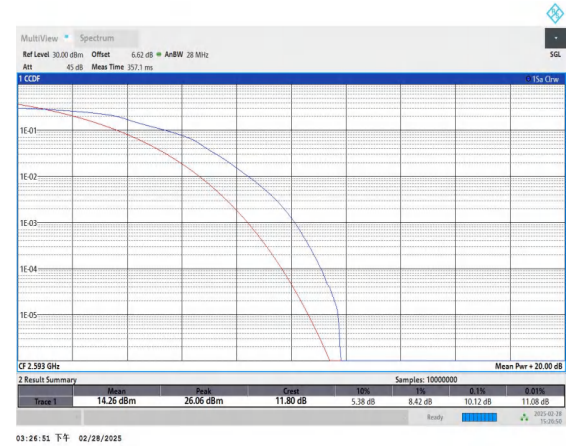
Band41-10MHz-16QAM-40620-50RB#0-PASS
