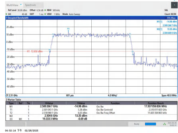
Band41-20MHz-16QAM-39790-100RB#0-PASS
