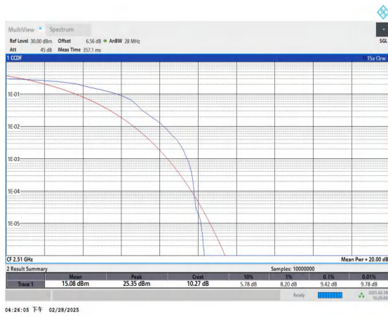
Band41-20MHz-16QAM-39790-1RB#0-PASS
