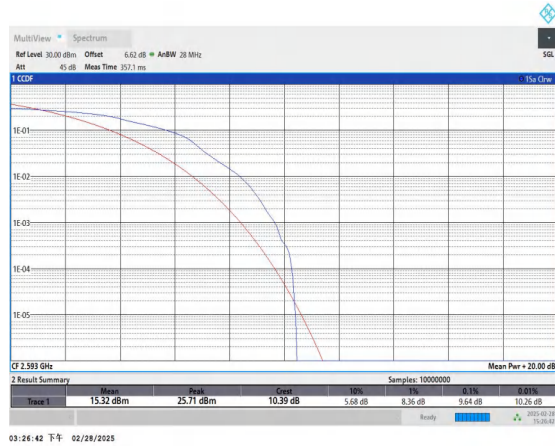
Band41-10MHz-16QAM-40620-1RB#0-PASS
