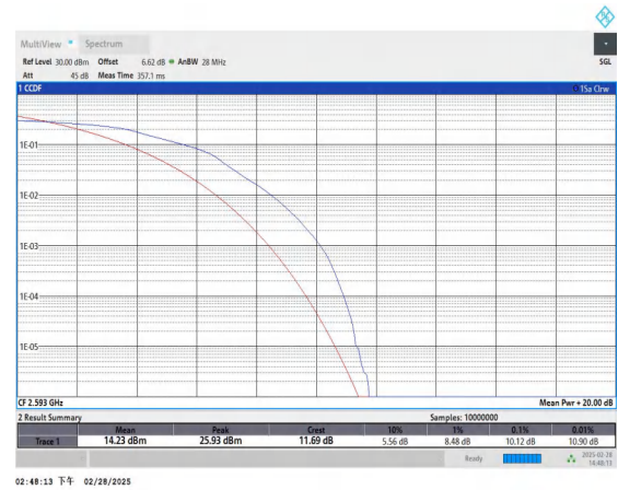
Band41-5MHz-16QAM-40620-25RB#0-PASS
