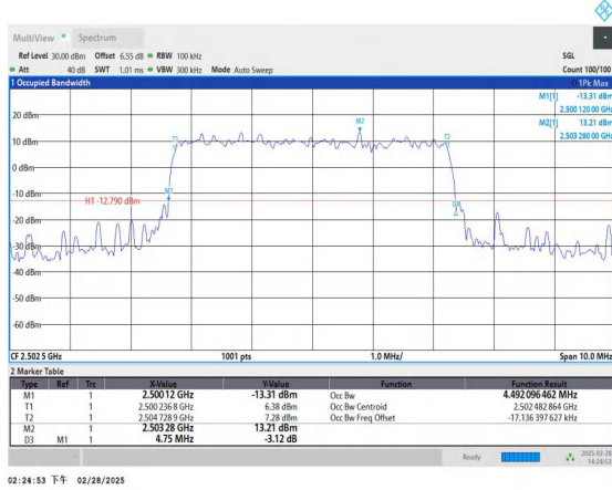
Band41-5MHz-QPSK-39715-25RB#0-PASS
