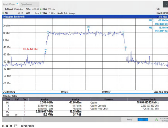
Band41-20MHz-16QAM-40620-100RB#0-PASS
