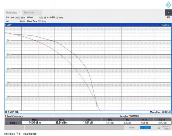
Band41-5MHz-16QAM-41565-25RB#0-PASS
