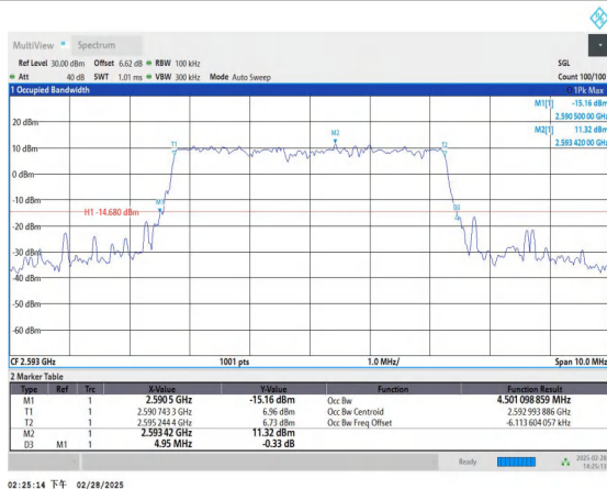
Band41-5MHz-16QAM-40620-25RB#0-PASS
