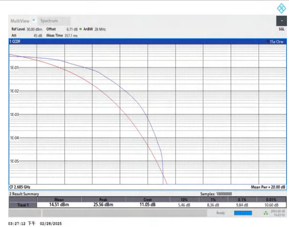
Band41-10MHz-16QAM-41540-50RB#0-PASS
