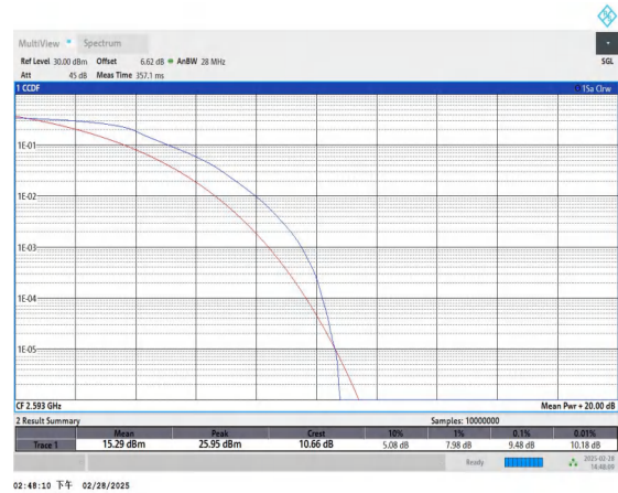
Band41-5MHz-QPSK-40620-25RB#0-PASS
