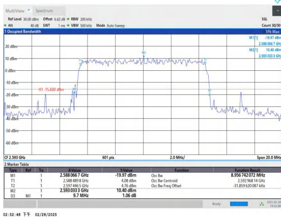
Band41-10MHz-16QAM-40620-50RB#0-PASS
