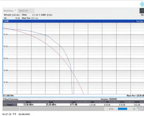
Band41-10MHz-16QAM-41540-1RB#0-PASS
