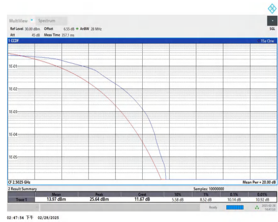
Band41-5MHz-16QAM-39715-25RB#0-PASS
