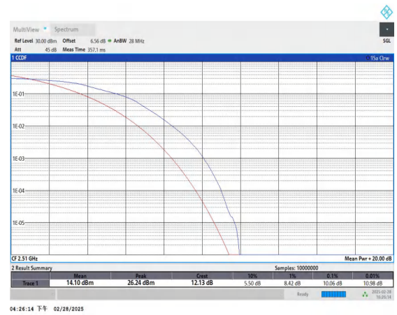
Band41-20MHz-16QAM-39790-100RB#0-PASS
