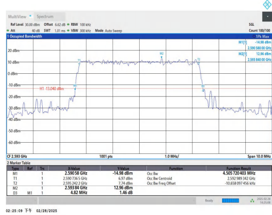
Band41-5MHz-QPSK-40620-25RB#0-PASS
