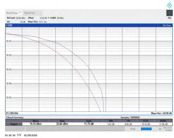
Band41-10MHz-16QAM-39740-50RB#0-PASS
