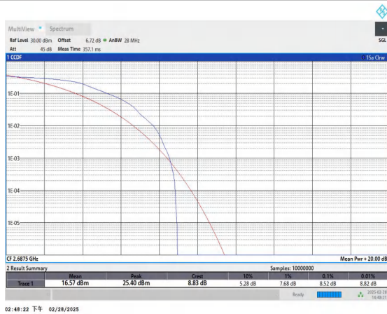
Band41-5MHz-QPSK-41565-1RB#0-PASS
