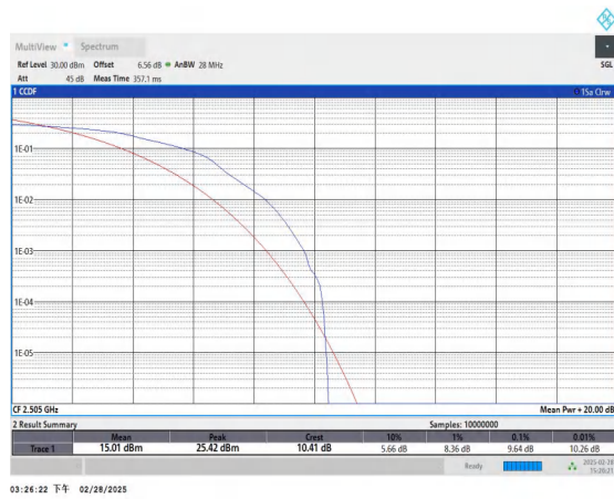
Band41-10MHz-16QAM-39740-1RB#0-PASS
