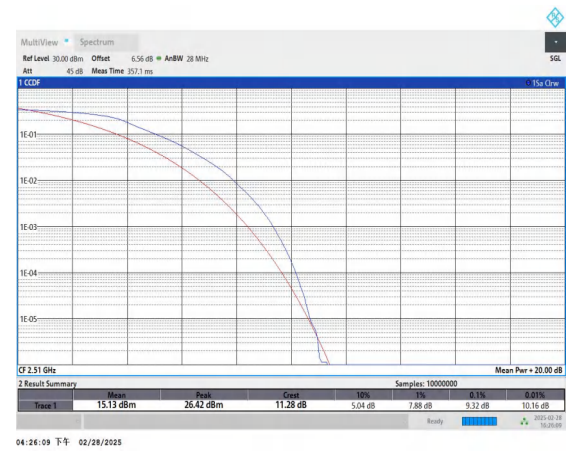
Band41-20MHz-QPSK-39790-100RB#0-PASS
