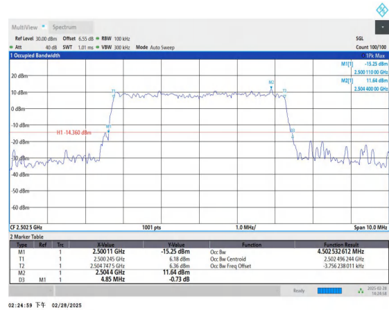
Band41-5MHz-16QAM-39715-25RB#0-PASS
