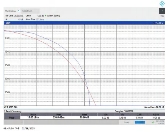
Band41-5MHz-QPSK-39715-25RB#0-PASS
