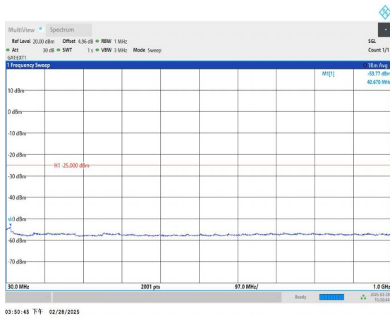
Band41_15MHz_QPSK_41515_1RB#0_30~1000_30~1000
