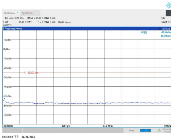
Band41_5MHz_QPSK_41565_1RB#0_30~1000_30~1000
