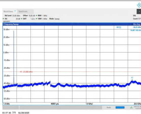
Band41_10MHz_16QAM_39740_1RB#0_1000~20000_1000~2000
