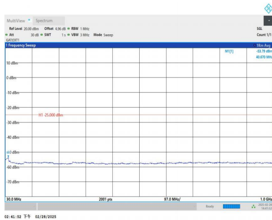
Band41_5MHz_16QAM_40620_1RB#0_30~1000_30~1000
