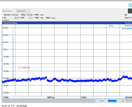
Band41_5MHz_QPSK_40620_1RB#0_1000~20000_1000~2000 0
