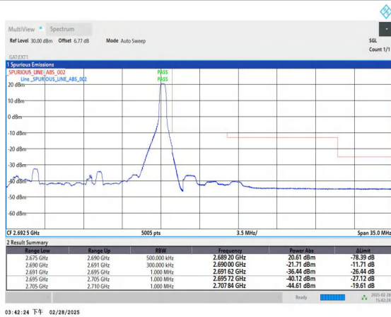
Band41_15MHz_QPSK_41515_1RB#74
