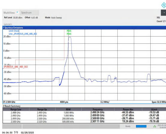
Band41_20MHz_16QAM_39790_1RB#0
