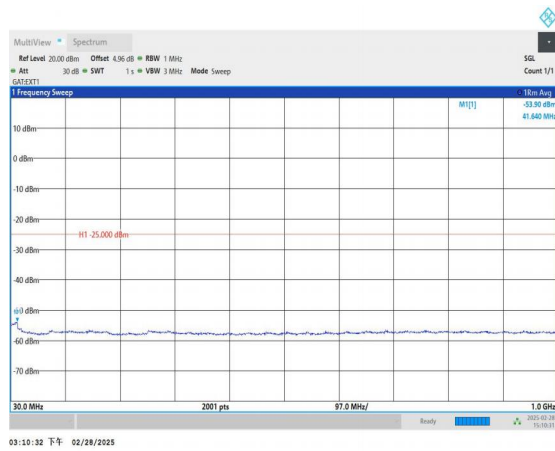
Band41_10MHz_QPSK_41540_1RB#0_30~1000_30~1000
