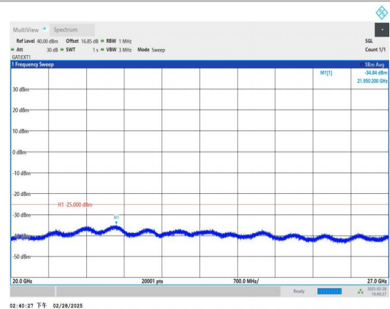
Band41_5MHz_16QAM_39715_1RB#0_20000~27000_20000~27000
