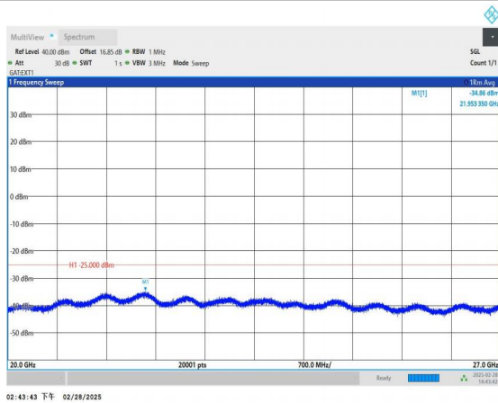
Band41_5MHz_QPSK_41565_1RB#0_20000~27000_20000~27000 000
