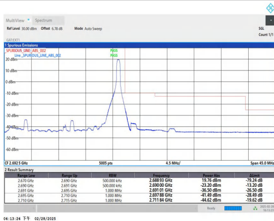
Band41_20MHz_16QAM_41490_1RB#99
