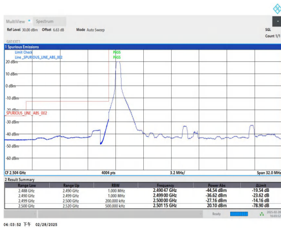
Band41_20MHz_QPSK_39790_1RB#0
