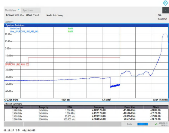
Band41_5MHz_QPSK_39715_1RB#24
