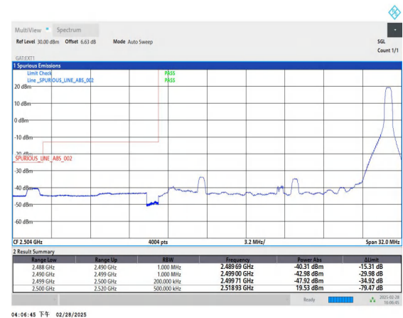
Band41_20MHz_16QAM_39790_1RB#99
