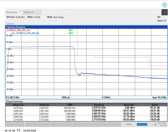
Band41_20MHz_16QAM_41490_100RB#0
