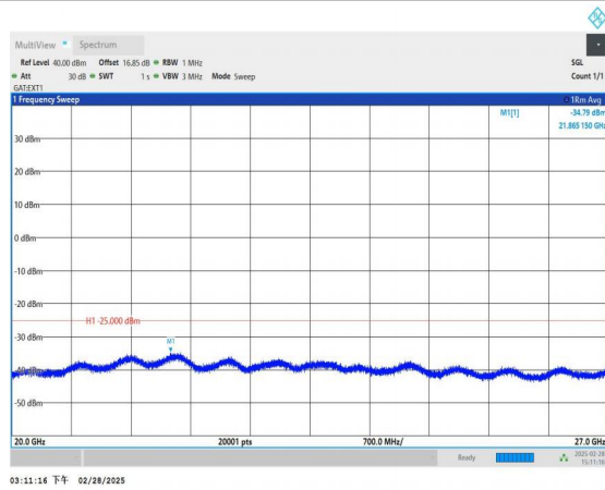
Band41_10MHz_QPSK_41540_1RB#0_20000~27000_20000~27000
