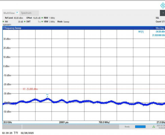
Band41_5MHz_QPSK_39715_1RB#0_20000~27000_20000~27000 000
