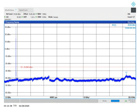
Band41_10MHz_QPSK_41540_1RB#0_1000~20000_1000~2000
