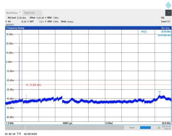
Band41_5MHz_16QAM_40620_1RB#0_1000~20000_1000~20000
