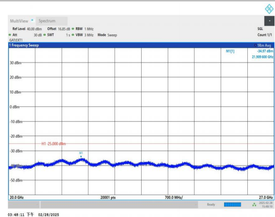
Band41_15MHz_16QAM_39765_1RB#0_20000~27000_20000~27000
