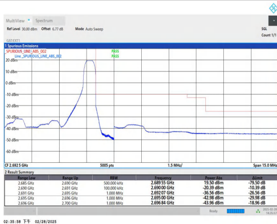
Band41_5MHz_16QAM_41565_1RB#24
