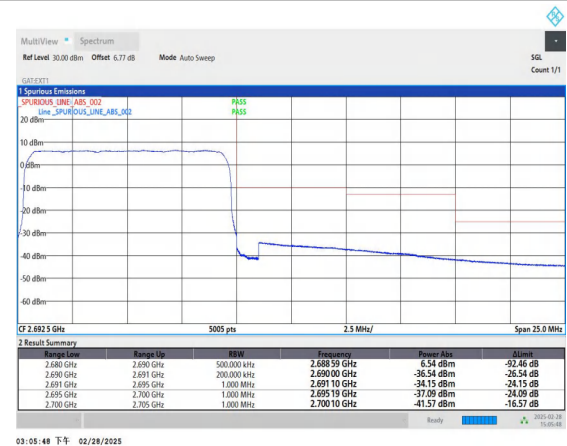
Band41_10MHz_16QAM_41540_50RB#0
