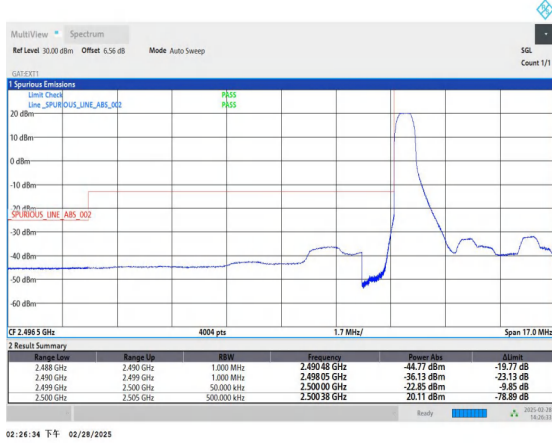
Band41_5MHz_QPSK_39715_1RB#0
