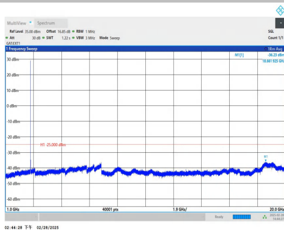
Band41_5MHz_16QAM_41565_1RB#0_1000~20000_1000~20000
