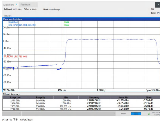
Band41_20MHz_16QAM_39790_100RB#0
