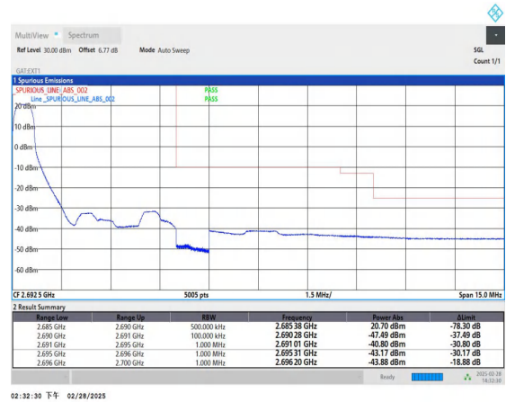
Band41_5MHz_QPSK_41565_1RB#0
