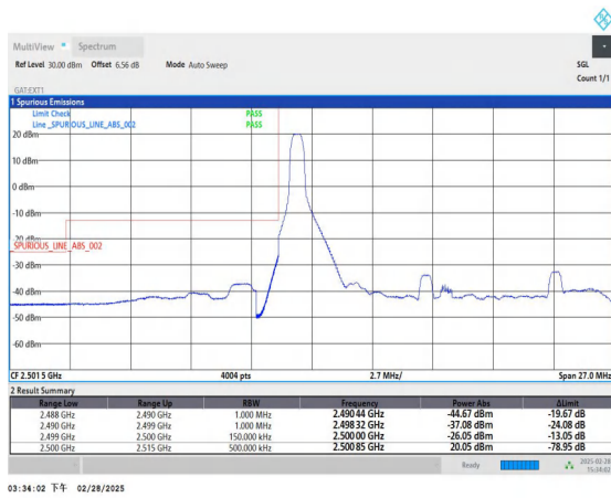
Band41_15MHz_QPSK_39765_1RB#0
