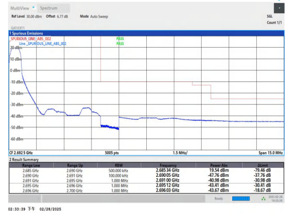
Band41_5MHz_16QAM_41565_1RB#0
