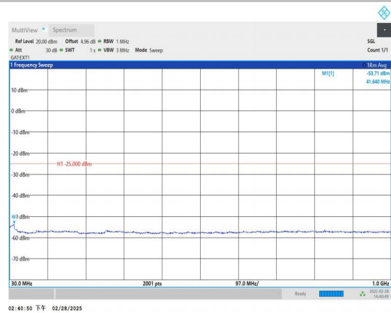
Band41_5MHz_QPSK_40620_1RB#0_30~1000_30~1000
