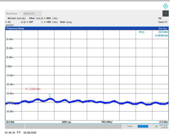
Band41_10MHz_16QAM_39740_1RB#0_20000~27000_20000~27000
