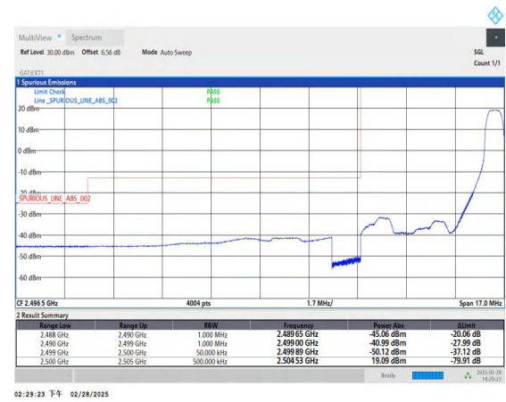
Band41_5MHz_16QAM_39715_1RB#24
