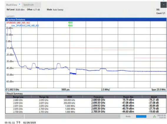
Band41_10MHz_16QAM_41540_1RB#0
