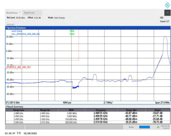
Band41_15MHz_QPSK_39765_1RB#74
