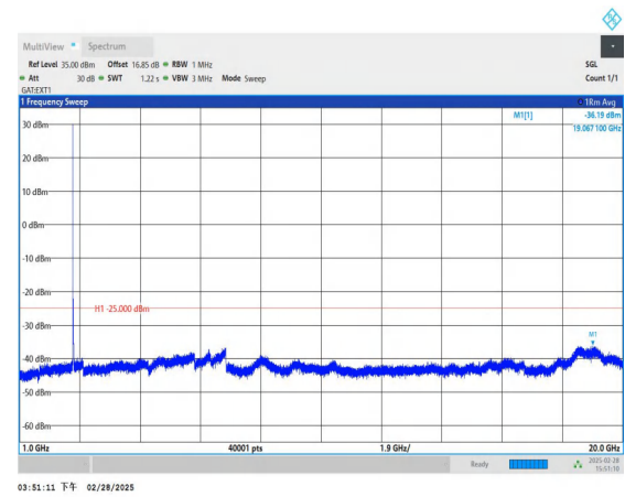
Band41_15MHz_QPSK_41515_1RB#0_1000~20000_1000~2000
