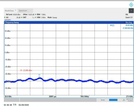
Band41_5MHz_16QAM_41565_1RB#0_20000~27000_20000~27000
