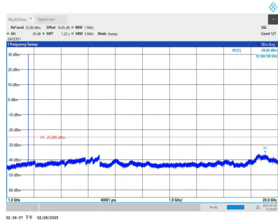
Band41_5MHz_QPSK_39715_1RB#0_1000~20000_1000~2000 0
