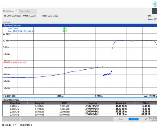
Band41_5MHz_QPSK_39715_25RB#0
