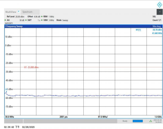
Band41_5MHz_16QAM_39715_1RB#0_30~1000_30~1000
