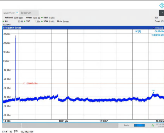
Band41_15MHz_16QAM_39765_1RB#0_1000~20000_1000~20000
