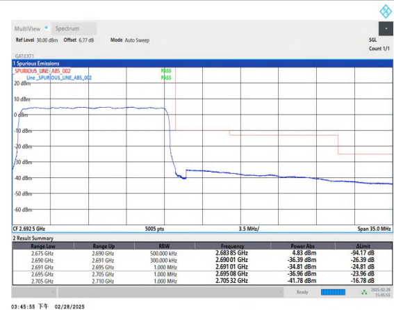
Band41_15MHz_16QAM_41515_75RB#0
