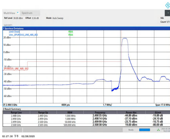
Band41_5MHz_16QAM_39715_1RB#0
