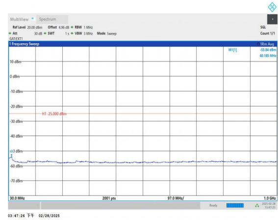
Band41_15MHz_16QAM_39765_1RB#0_30~1000_30~1000
