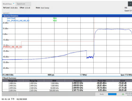
Band41_5MHz_16QAM_39715_25RB#0
