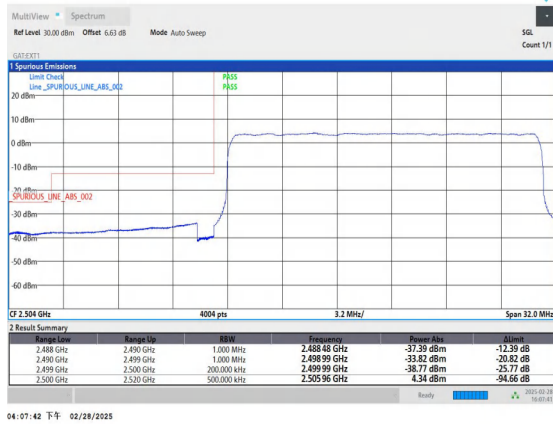
Band41_20MHz_QPSK_39790_100RB#0
