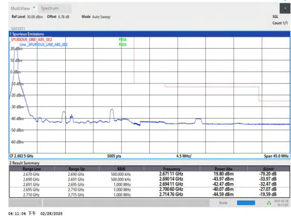
Band41_20MHz_16QAM_41490_1RB#0
