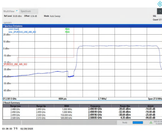
Band41_15MHz_16QAM_39765_75RB#0
