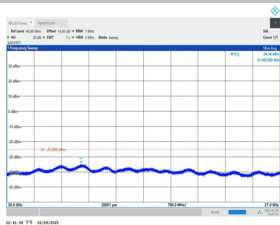
Band41_5MHz_QPSK_40620_1RB#0_20000~27000_20000~27000 000
