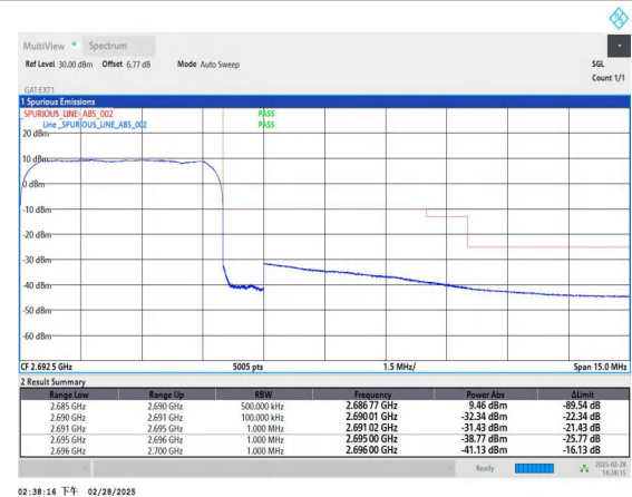
Band41_5MHz_16QAM_41565_25RB#0
