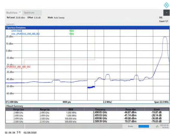
Band41_10MHz_16QAM_39740_1RB#49
