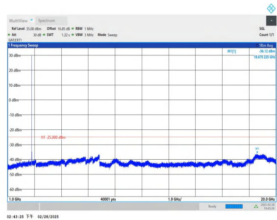
Band41_5MHz_QPSK_41565_1RB#0_1000~20000_1000~2000 0
