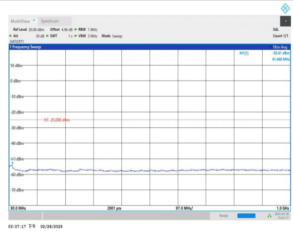
Band41_10MHz_16QAM_39740_1RB#0_30~1000_30~1000
