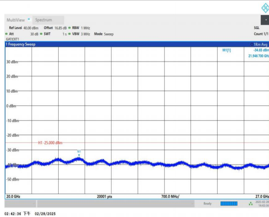
Band41_5MHz_16QAM_40620_1RB#0_20000~27000_20000~27000
