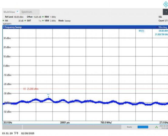
Band41_15MHz_QPSK_41515_1RB#0_20000~27000_20000~27000
