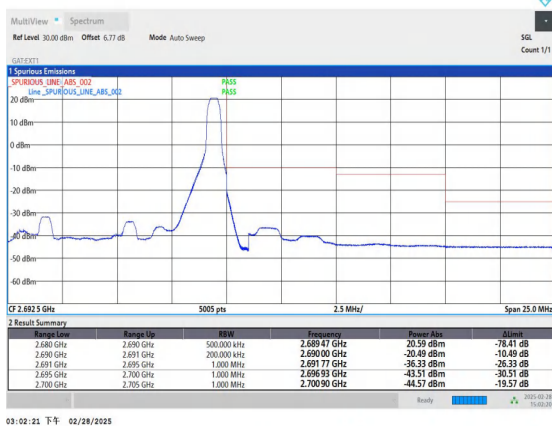
Band41_10MHz_QPSK_41540_1RB#49
