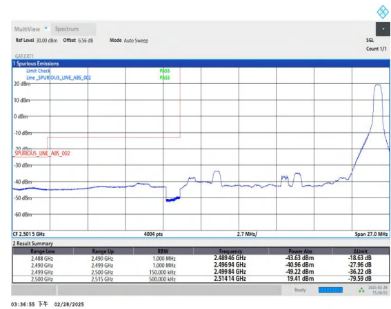
Band41_15MHz_16QAM_39765_1RB#74
