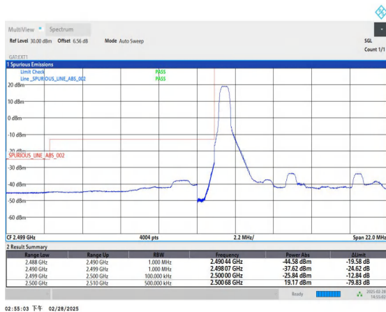
Band41_10MHz_16QAM_39740_1RB#0
