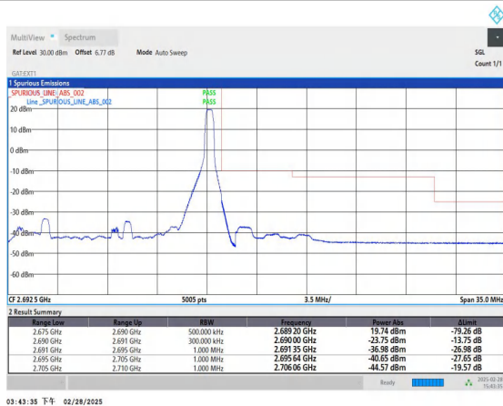
Band41_15MHz_16QAM_41515_1RB#74
