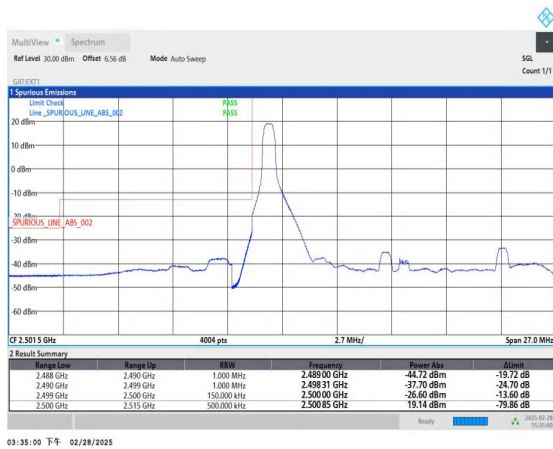
Band41_15MHz_16QAM_39765_1RB#0
