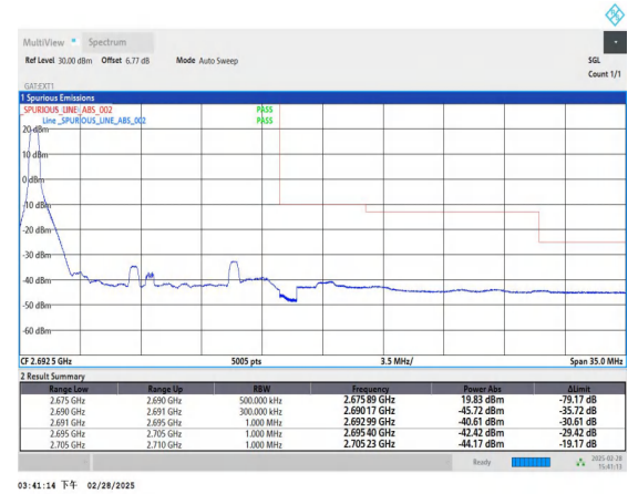
Band41_15MHz_16QAM_41515_1RB#0
