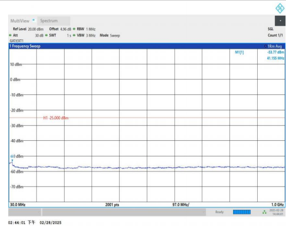
Band41_5MHz_16QAM_41565_1RB#0_30~1000_30~1000
