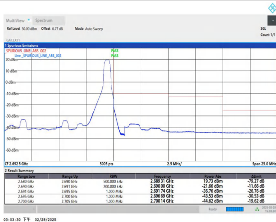
Band41_10MHz_16QAM_41540_1RB#49
