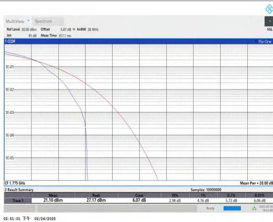
Band66-10MHz-16QAM-132622-1RB#0-PASS
