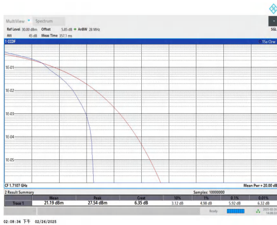
Band66-1.4MHz-16QAM-131979-1RB#0-PASS
