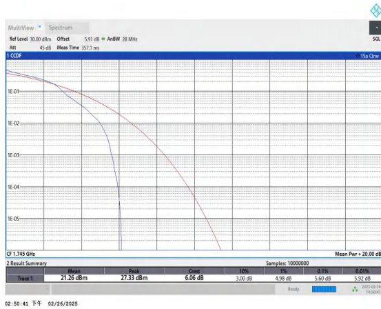
Band66-10MHz-16QAM-132322-1RB#0-PASS
