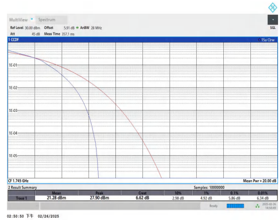
Band66-10MHz-16QAM-132322-50RB#0-PASS
