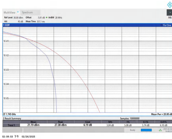
Band66-1.4MHz-16QAM-132322-1RB#0-PASS
