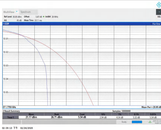
Band66-1.4MHz-16QAM-132665-1RB#0-PASS
