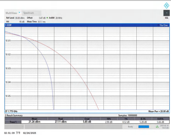
Band66-10MHz-16QAM-132622-50RB#0-PASS
