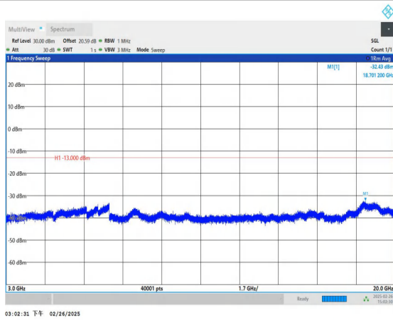
Band66_15MHz_QPSK_132597_1RB#0_3000~20000_3000~20
