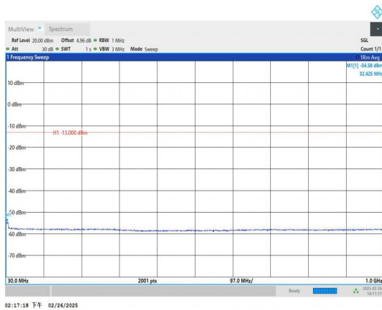
Band66_3MHz_QPSK_131987_1RB#0_30~1000_30~1000
