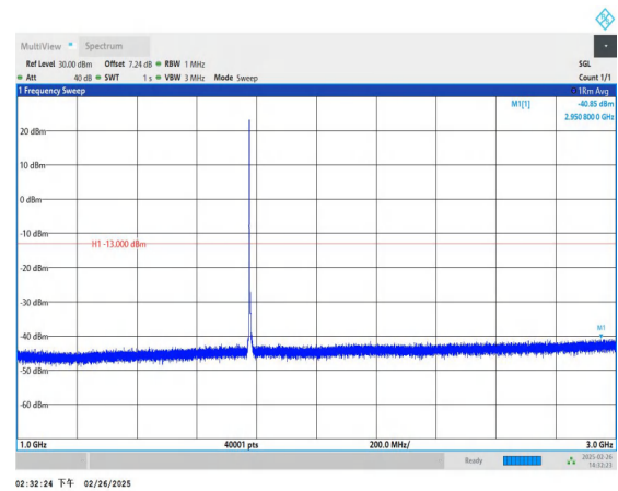
Band66_5MHz_QPSK_132647_1RB#0_1000~3000_1000~3000
