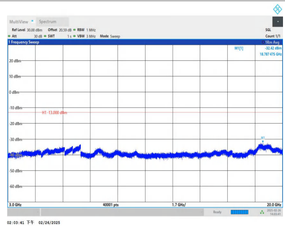
Band66_1.4MHz_16QAM_131979_1RB#0_3000~20000_3000~20000
