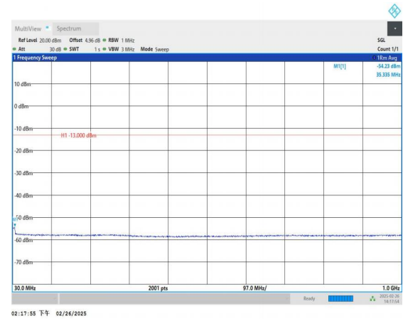
Band66_3MHz_QPSK_132322_1RB#0_30~1000_30~1000
