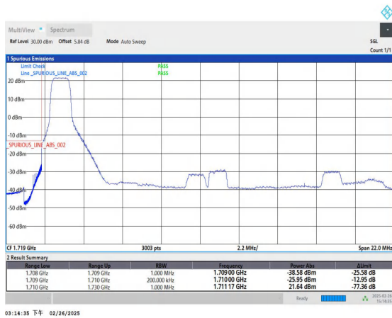
Band66_20MHz_16QAM_132072_1RB#0
