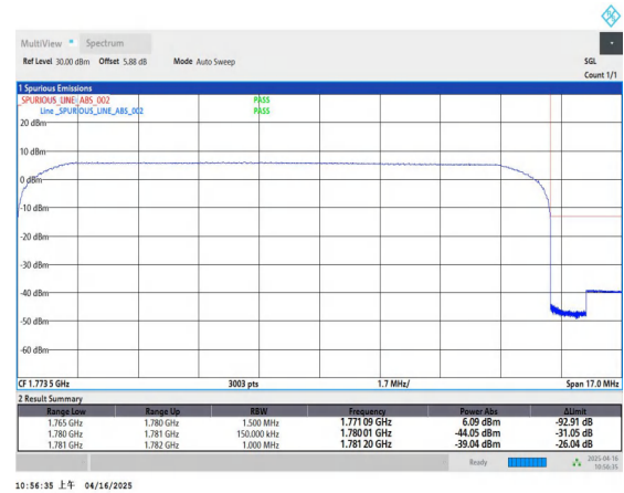
Band66_15MHz_16QAM_132597_75RB#0
