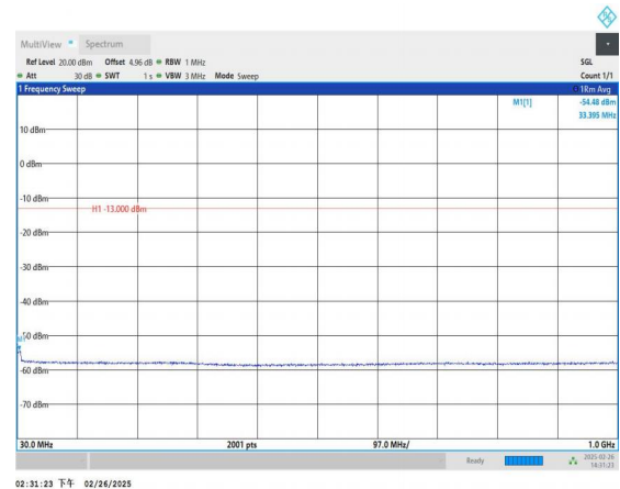
Band66_5MHz_16QAM_131997_1RB#0_30~1000_30~1000
