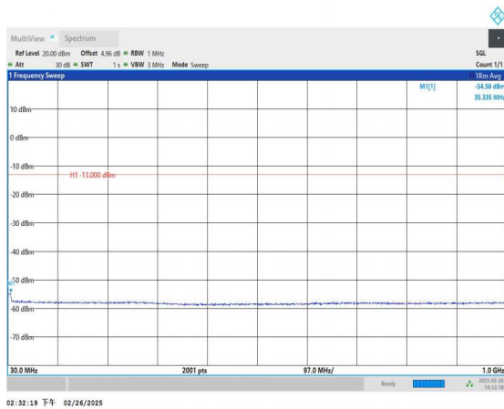
Band66_5MHz_QPSK_132647_1RB#0_30~1000_30~1000
