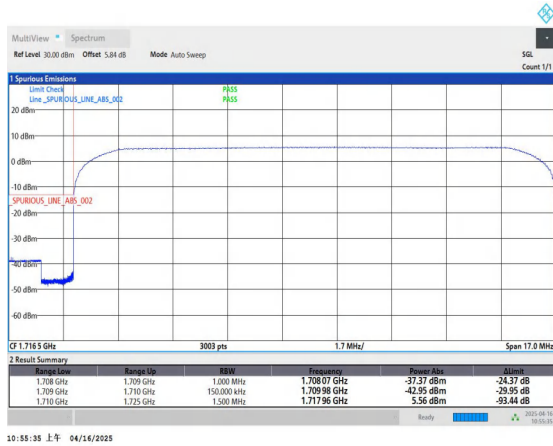
Band66_15MHz_16QAM_132047_75RB#0
