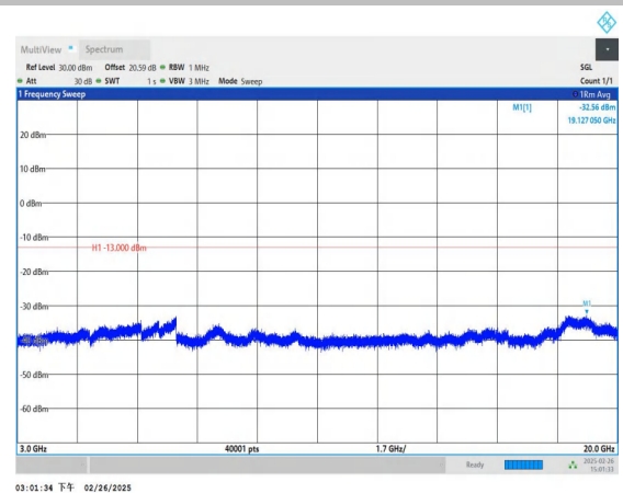
Band66_15MHz_16QAM_132047_1RB#0_3000~20000_3000~20000
