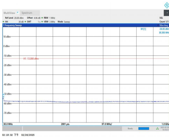
Band66_3MHz_QPSK_132657_1RB#0_30~1000_30~1000
