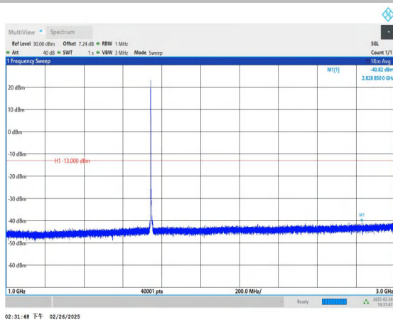
Band66_5MHz_QPSK_132322_1RB#0_1000~3000_1000~3000
