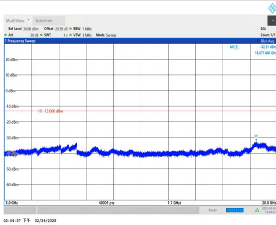
Band66_1.4MHz_QPSK_132665_1RB#0_3000~20000_3000~20000
