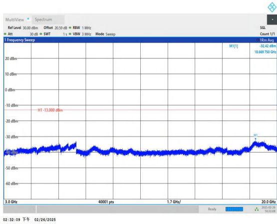
Band66_5MHz_16QAM_132322_1RB#0_3000~20000_3000~20000
