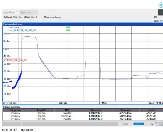
Band66_15MHz_16QAM_132047_1RB#0
