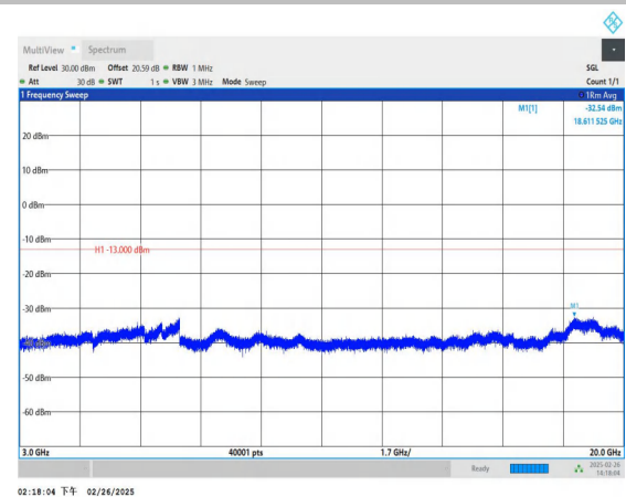
Band66_3MHz_QPSK_132322_1RB#0_3000~20000_3000~20000
