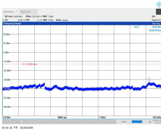
Band66_5MHz_QPSK_131997_1RB#0_3000~20000_3000~2000
