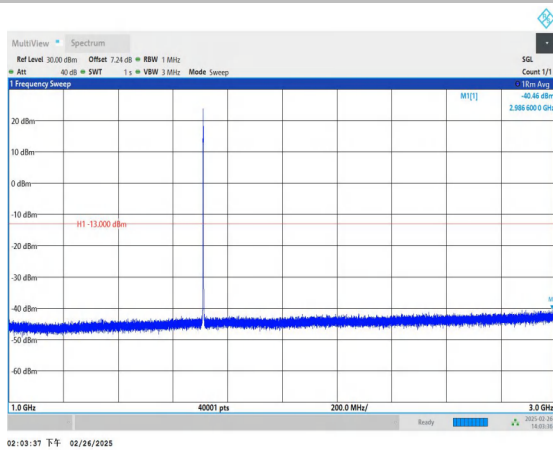
Band66_1.4MHz_16QAM_131979_1RB#0_1000~3000_1000~3000
