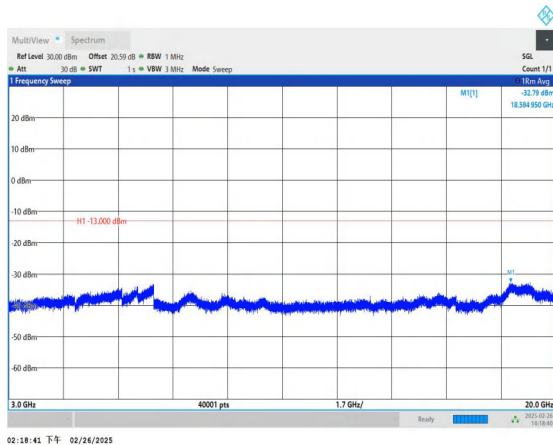
Band66_3MHz_QPSK_132657_1RB#0_3000~20000_3000~2000
