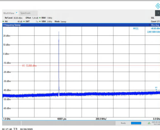
Band66_3MHz_16QAM_131987_1RB#0_1000~3000_1000~3000
