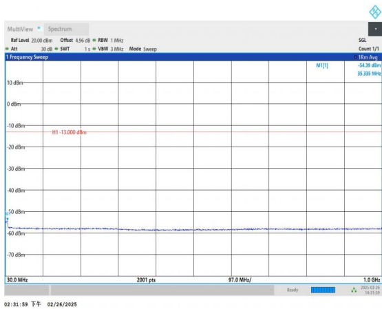
Band66_5MHz_16QAM_132322_1RB#0_30~1000_30~1000
