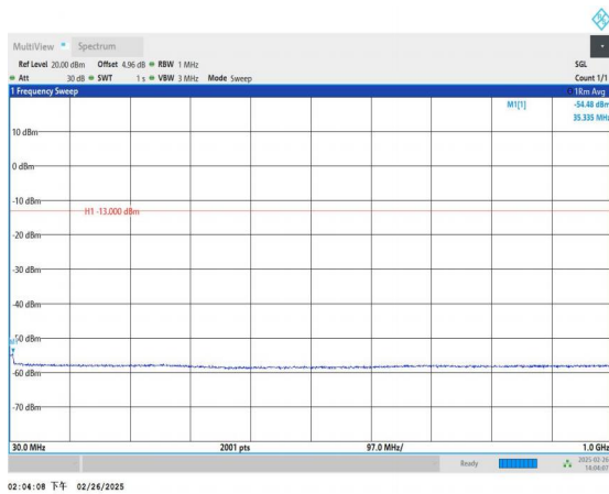
Band66_1.4MHz_16QAM_132322_1RB#0_30~1000_30~1000
