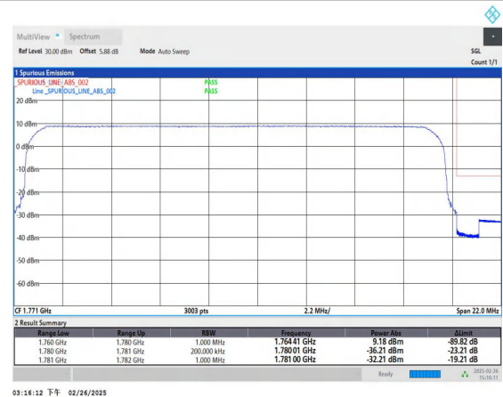
Band66_20MHz_QPSK_132572_100RB#0
