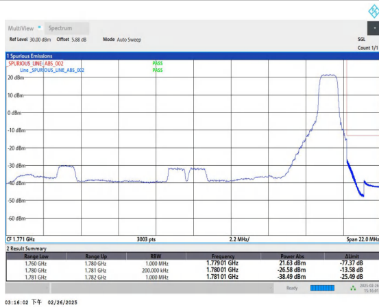
Band66_20MHz_16QAM_132572_1RB#99
