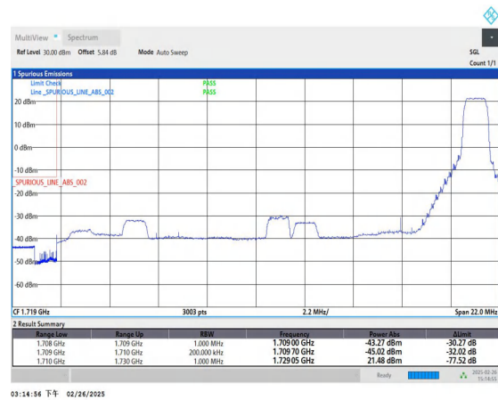
Band66_20MHz_16QAM_132072_1RB#99
