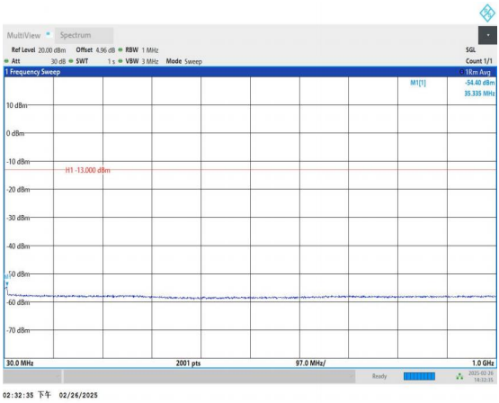
Band66_5MHz_16QAM_132647_1RB#0_30~1000_30~1000
