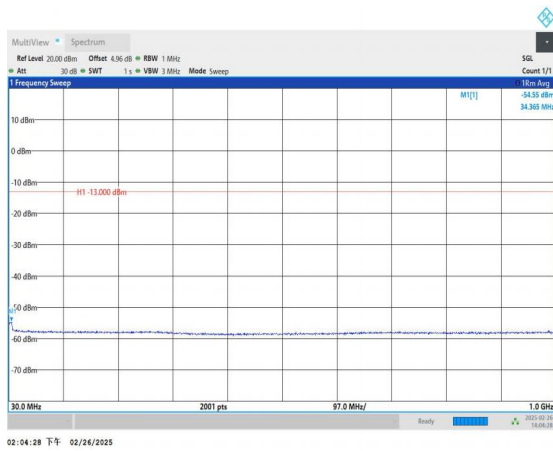
Band66_1.4MHz_QPSK_132665_1RB#0_30~1000_30~1000
