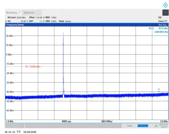
Band66_5MHz_QPSK_131997_1RB#0_1000~3000_1000~3000
