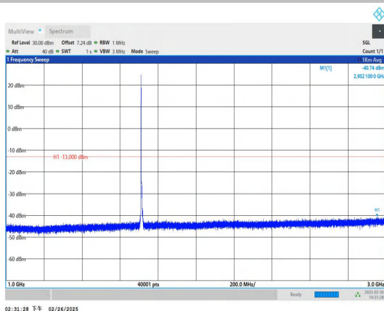
Band66_5MHz_16QAM_131997_1RB#0_1000~3000_1000~3000
