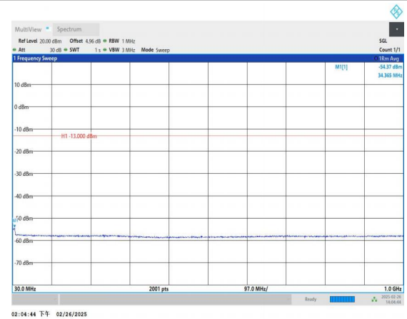
Band66_1.4MHz_16QAM_132665_1RB#0_30~1000_30~1000
