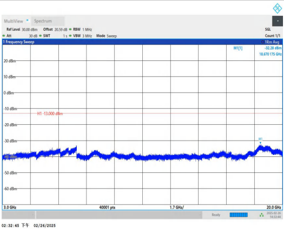
Band66_5MHz_16QAM_132647_1RB#0_3000~20000_3000~20000
