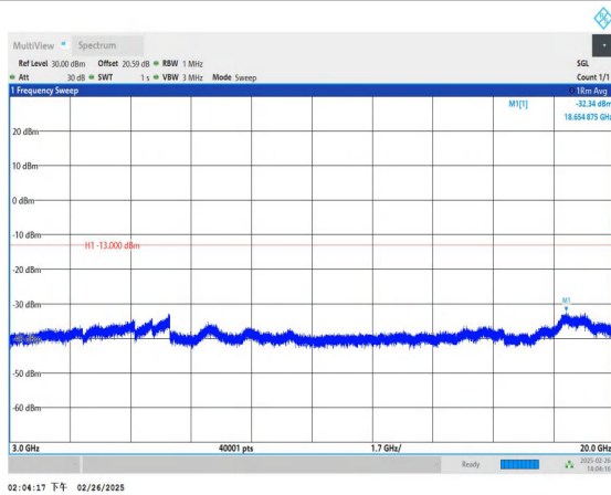
Band66_1.4MHz_16QAM_132322_1RB#0_3000~20000_3000~20000
