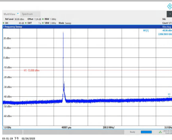
Band66_15MHz_16QAM_132047_1RB#0_1000~3000_1000~3
