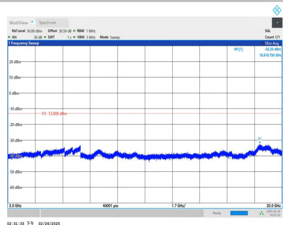
Band66_5MHz_16QAM_131997_1RB#0_3000~20000_3000~20000
