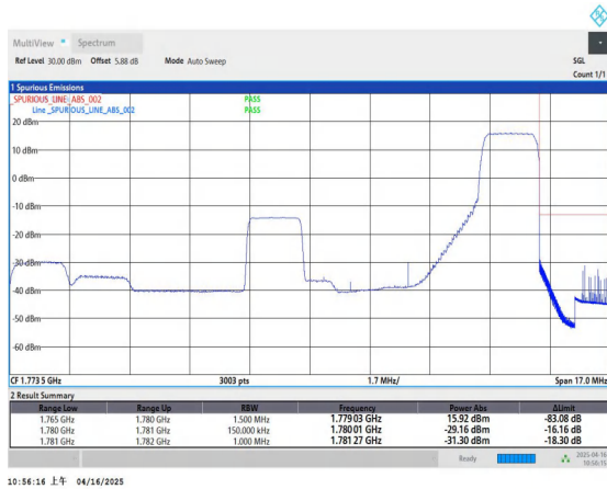
Band66_15MHz_16QAM_132597_1RB#74
