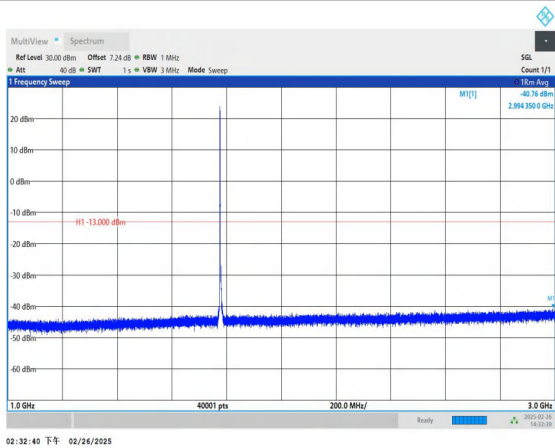
Band66_5MHz_16QAM_132647_1RB#0_1000~3000_1000~3000
