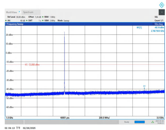
Band66_1.4MHz_16QAM_132322_1RB#0_1000~3000_1000~3000
