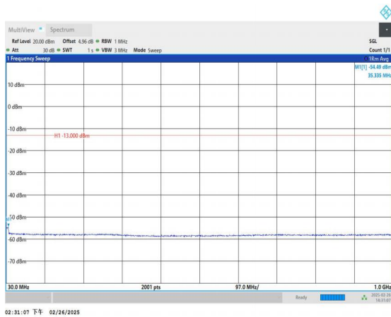
Band66_5MHz_QPSK_131997_1RB#0_30~1000_30~1000
