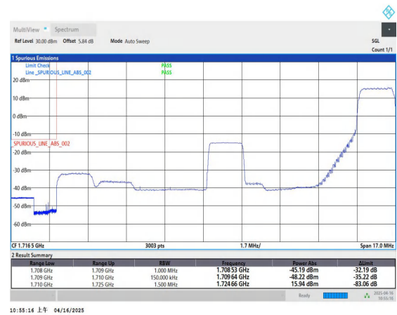
Band66_15MHz_16QAM_132047_1RB#74
