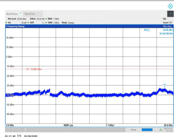
Band66_3MHz_16QAM_131987_1RB#0_3000~20000_3000~20000
