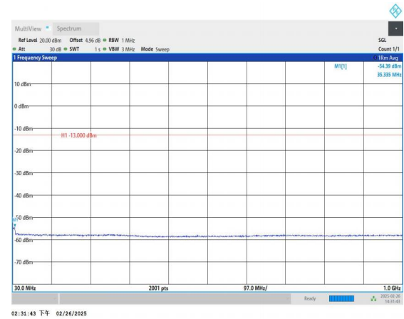
Band66_5MHz_QPSK_132322_1RB#0_30~1000_30~1000
