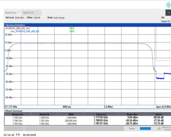
Band66_20MHz_16QAM_132572_100RB#0
