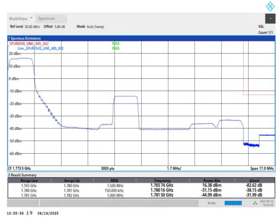
Band66_15MHz_16QAM_132597_1RB#0
