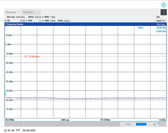
Band66_15MHz_16QAM_132047_1RB#0_30~1000_30~1000
