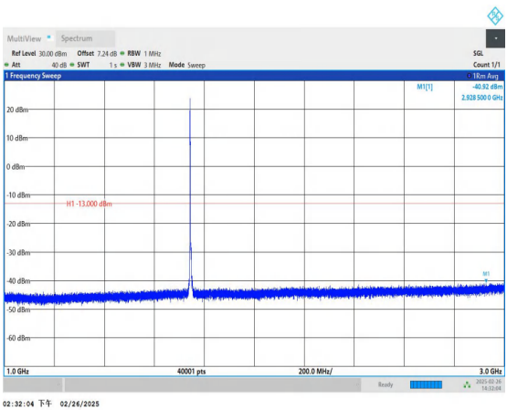
Band66_5MHz_16QAM_132322_1RB#0_1000~3000_1000~3000
