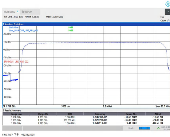
Band66_20MHz_16QAM_132072_100RB#0
