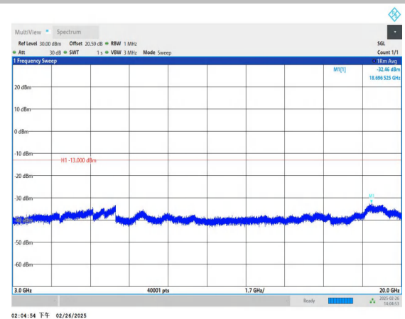
Band66_1.4MHz_16QAM_132665_1RB#0_3000~20000_3000~20000
