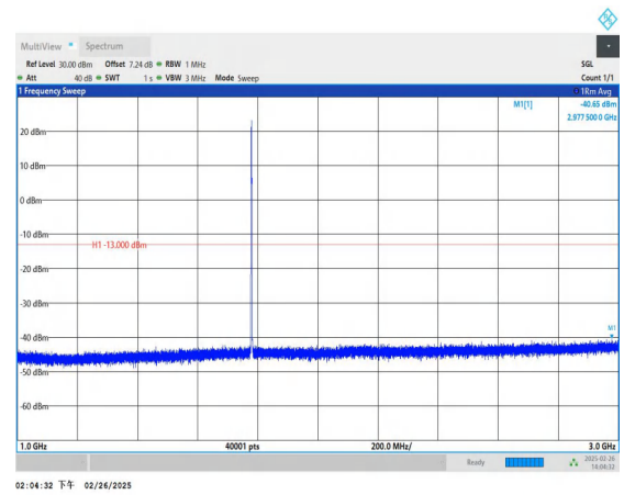
Band66_1.4MHz_QPSK_132665_1RB#0_1000~3000_1000~3000
