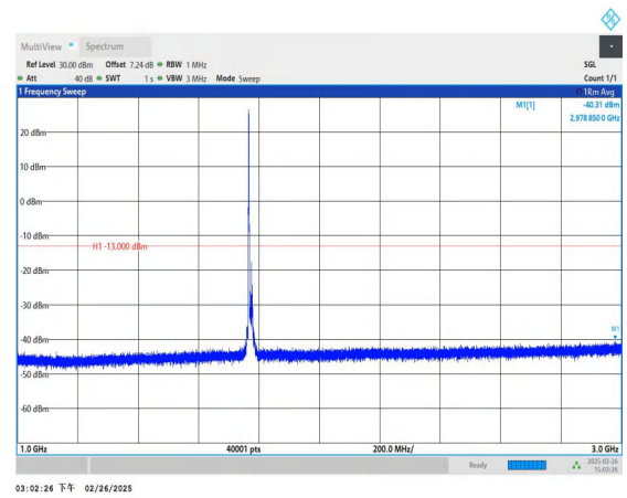
Band66_15MHz_QPSK_132597_1RB#0_1000~3000_1000~300
