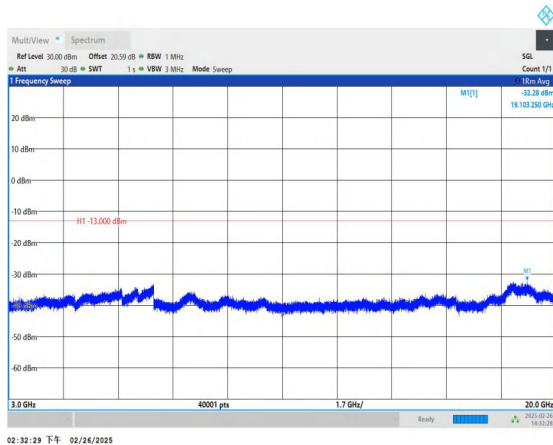
Band66_5MHz_QPSK_132647_1RB#0_3000~20000_3000~20000
