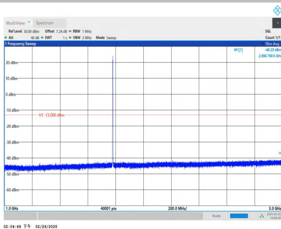
Band66_1.4MHz_16QAM_132665_1RB#0_1000~3000_1000~3000
