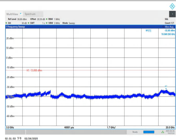
Band66_5MHz_QPSK_132322_1RB#0_3000~20000_3000~2000
