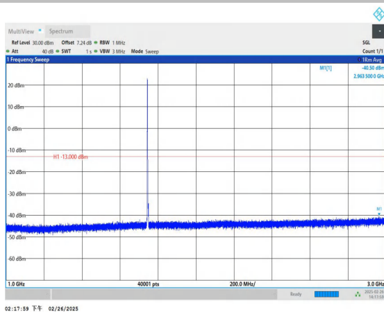
Band66_3MHz_QPSK_132322_1RB#0_1000~3000_1000~3000
