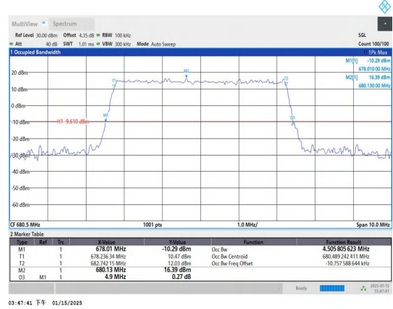
Band71-5MHz-QPSK-133297-25RB#0-PASS
