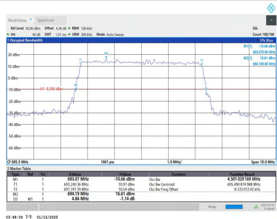
Band71-5MHz-16QAM-133447-25RB#0-PASS
