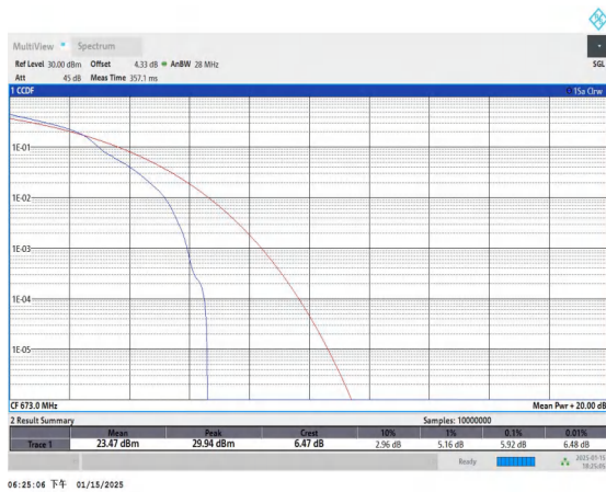
Band71-20MHz-16QAM-133222-1RB#0-PASS
