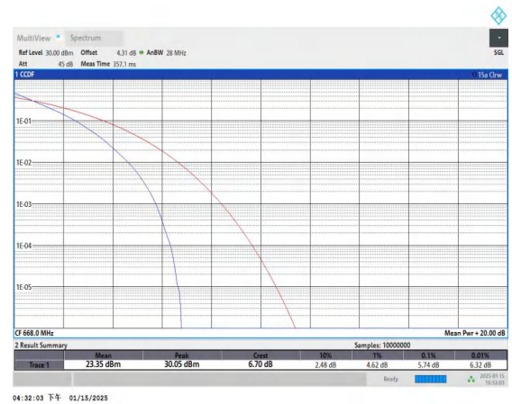
Band71-10MHz-QPSK-133172-50RB#0-PASS
