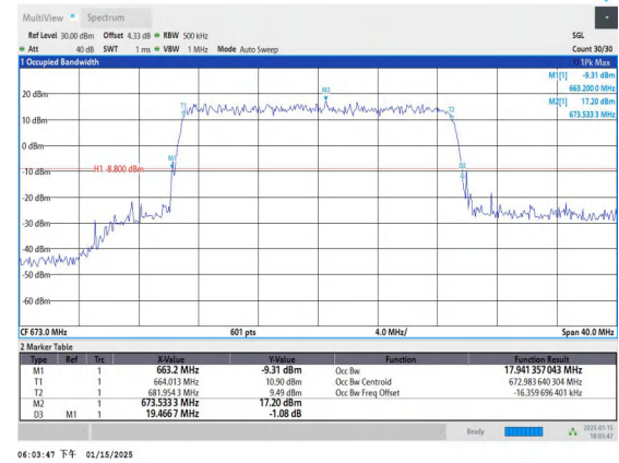
Band71-20MHz-16QAM-133222-100RB#0-PASS
