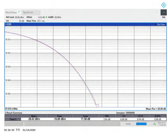
Band71-15MHz-16QAM-133197-75RB#0-PASS
