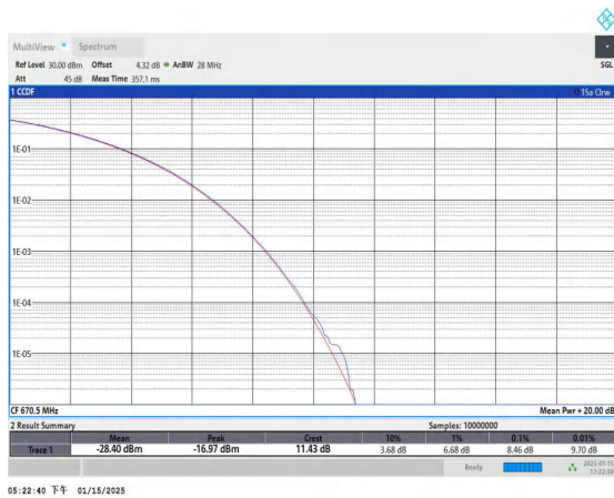
Band71-15MHz-16QAM-133197-1RB#0-PASS
