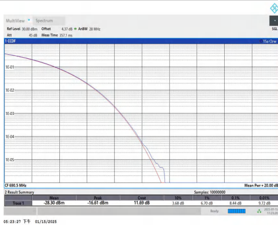
Band71-15MHz-QPSK-133397-1RB#0-PASS
