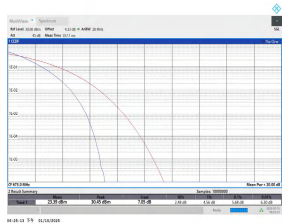
Band71-20MHz-QPSK-133222-100RB#0-PASS
