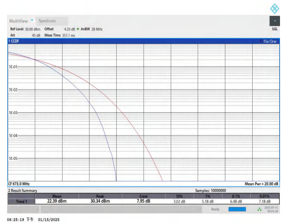
Band71-20MHz-16QAM-133222-100RB#0-PASS
