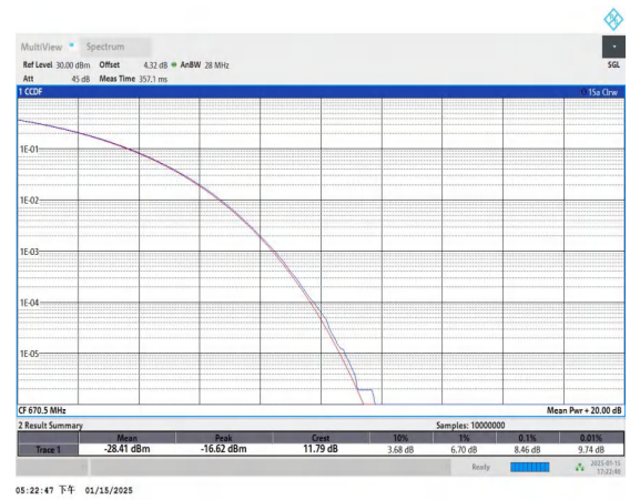
Band71-15MHz-QPSK-133197-75RB#0-PASS
