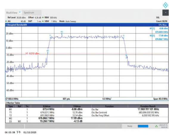
Band71-20MHz-QPSK-133322-100RB#0-PASS
