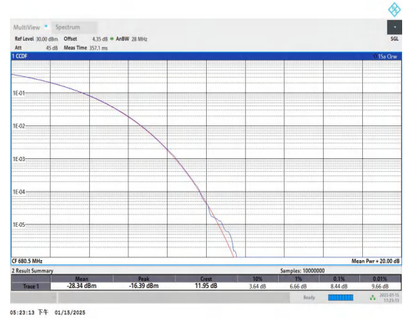
Band71-15MHz-QPSK-133297-75RB#0-PASS
