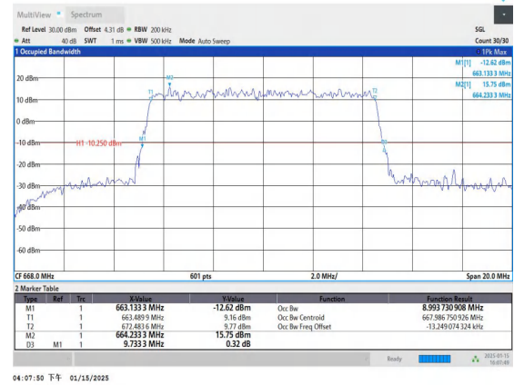
Band71-10MHz-16QAM-133172-50RB#0-PASS
