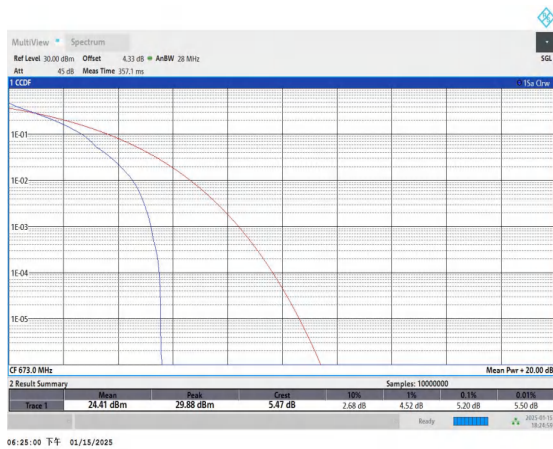
Band71-20MHz-QPSK-133222-1RB#0-PASS
