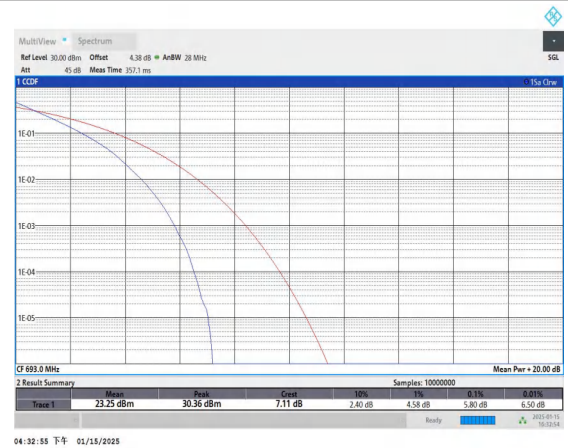
Band71-10MHz-QPSK-133422-50RB#0-PASS
