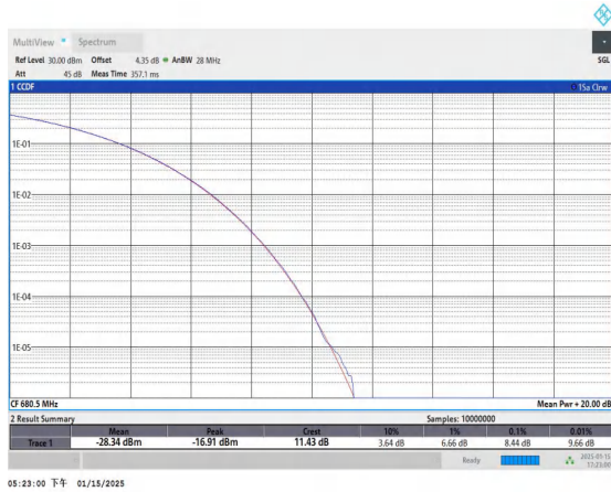
Band71-15MHz-QPSK-133297-1RB#0-PASS
