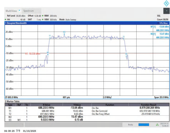
Band71-10MHz-16QAM-133422-50RB#0-PASS
