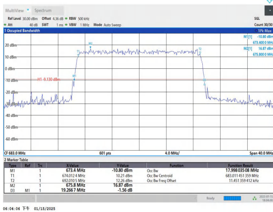
Band71-20MHz-16QAM-133322-100RB#0-PASS
