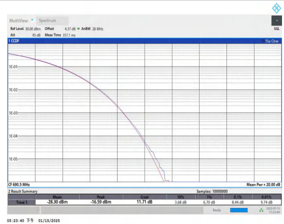
Band71-15MHz-QPSK-133397-75RB#0-PASS
