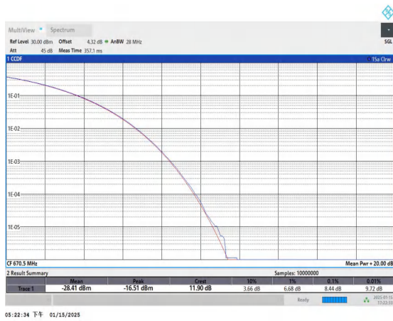
Band71-15MHz-QPSK-133197-1RB#0-PASS
