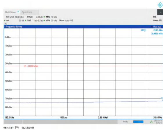
Band2-9538-0.15~30MHz-PASS
