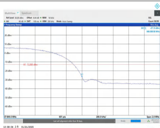
Band5-4233-PASS
