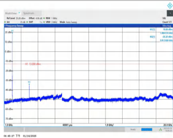
Band2-9538-1000~20000MHz-PASS
