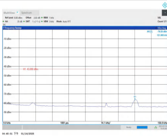
Band2-9538-0.009~0.15MHz-PASS
