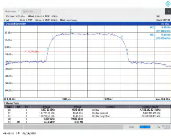
Band2-9400-PASS
