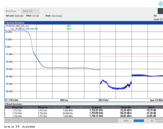
Band4_3MHz_16QAM_20385_1RB#0
