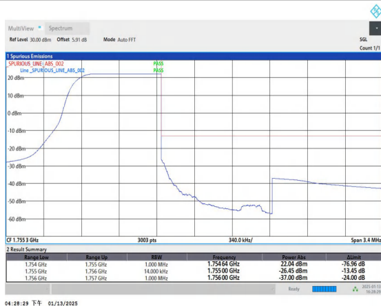
Band4_1.4MHz_QPSK_20393_1RB#5
