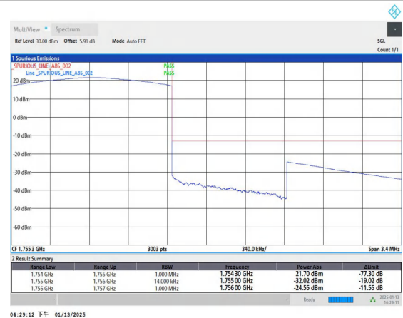
Band4_1.4MHz_16QAM_20393_6RB#0
