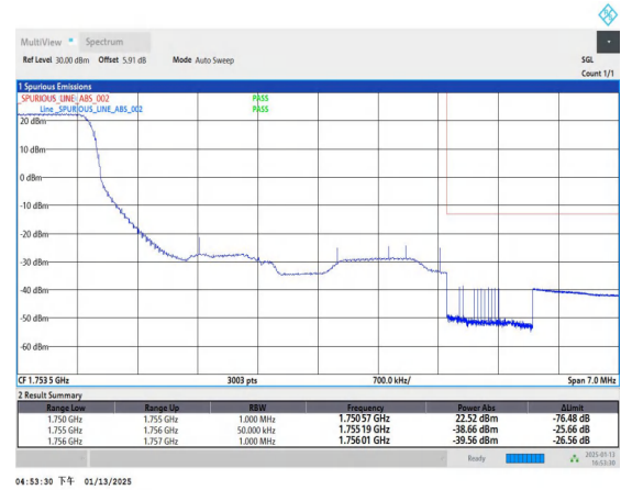
Band4_5MHz_16QAM_20375_1RB#0
