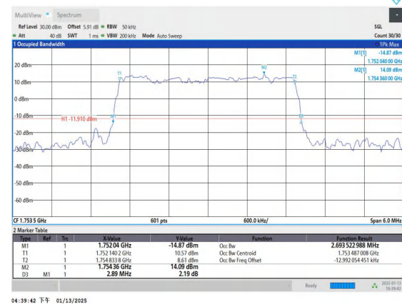
Band4-3MHz-16QAM-20385-15RB#0-PASS
