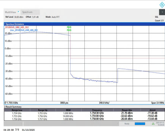
Band4_1.4MHz_QPSK_20393_6RB#0
