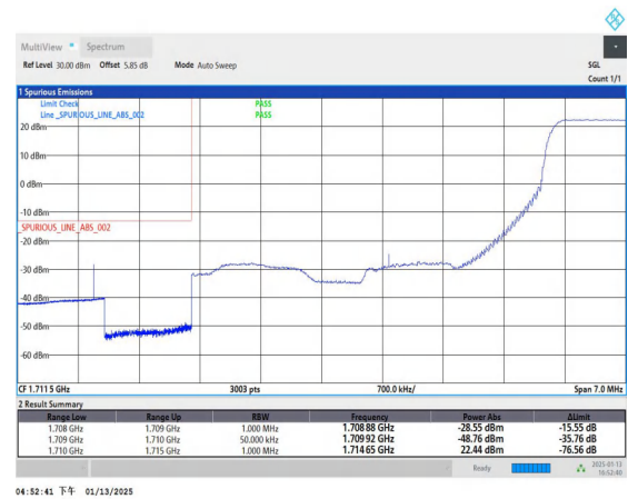
Band4_5MHz_QPSK_19975_1RB#24
