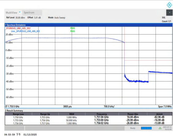
Band4_5MHz_QPSK_20375_25RB#0
