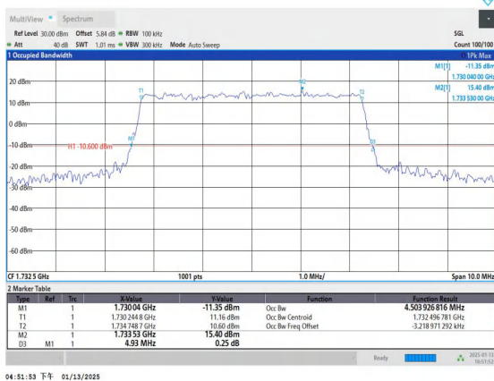
Band4-5MHz-16QAM-20175-25RB#0-PASS
