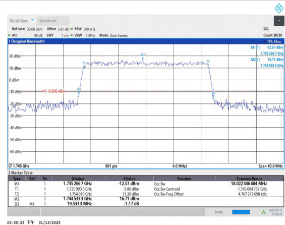
Band4-20MHz-16QAM-20300-100RB#0-PASS
