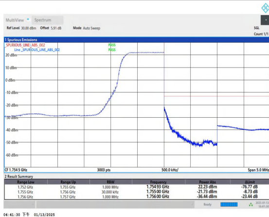
Band4_3MHz_16QAM_20385_1RB#14
