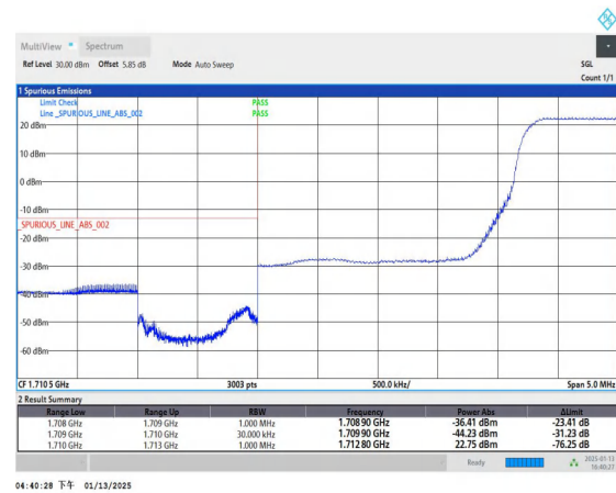
Band4_3MHz_16QAM_19965_1RB#14
