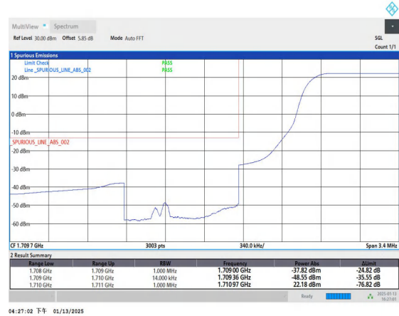
Band4_1.4MHz_QPSK_19957_1RB#5
