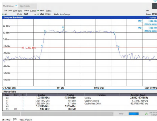
Band4-3MHz-16QAM-20175-15RB#0-PASS
