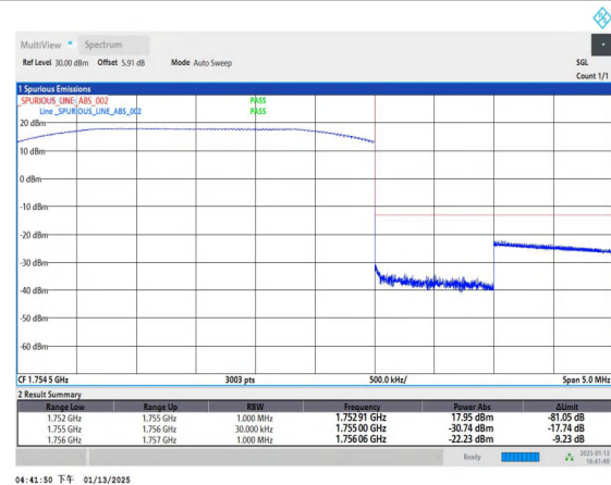
Band4_3MHz_16QAM_20385_15RB#0
