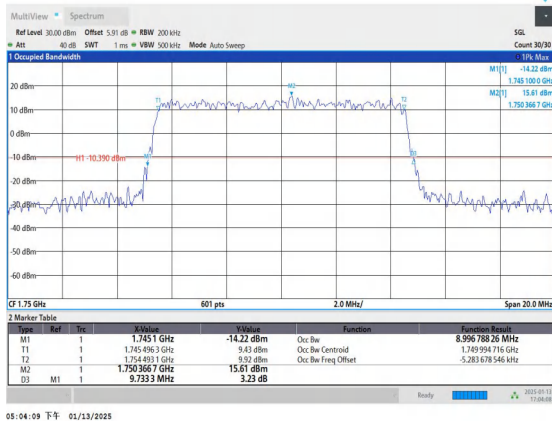
Band4-10MHz-QPSK-20350-50RB#0-PASS
