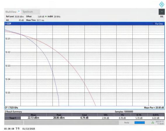
Band4-20MHz-16QAM-20175-100RB#0-PASS
