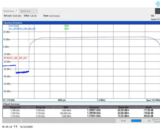
Band4_10MHz_16QAM_20000_50RB#0
