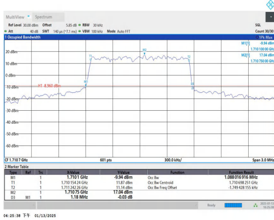
Band4-1.4MHz-QPSK-19957-6RB#0-PASS
