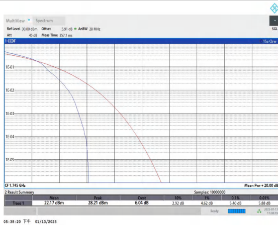
Band4-20MHz-16QAM-20300-1RB#0-PASS
