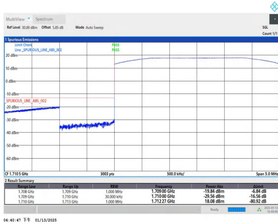
Band4_3MHz_16QAM_19965_15RB#0
