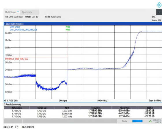
Band4_3MHz_QPSK_19965_1RB#14
