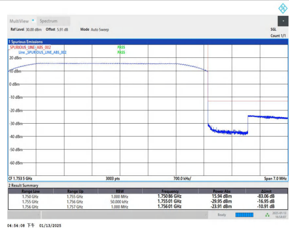
Band4_5MHz_16QAM_20375_25RB#0
