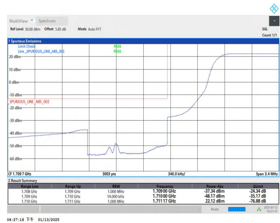
Band4_1.4MHz_16QAM_19957_1RB#5
