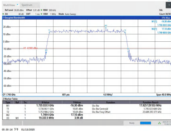
Band4-20MHz-QPSK-20300-100RB#0-PASS
