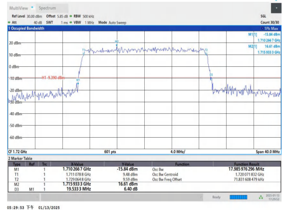
Band4-20MHz-16QAM-20050-100RB#0-PASS
