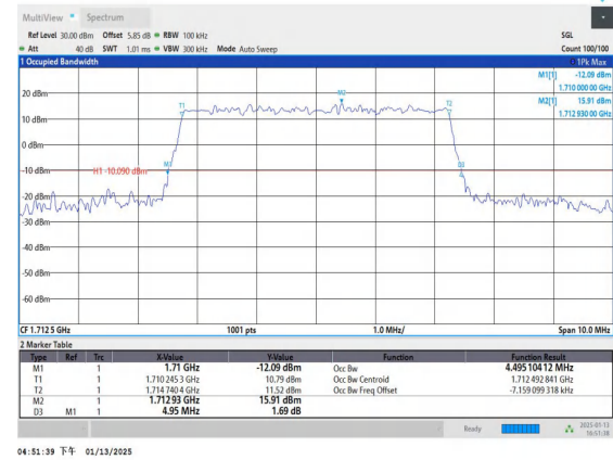
Band4-5MHz-16QAM-19975-25RB#0-PASS
