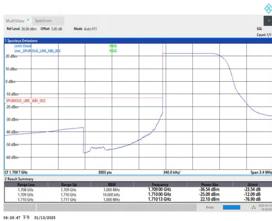
Band4_1.4MHz_16QAM_19957_1RB#0
