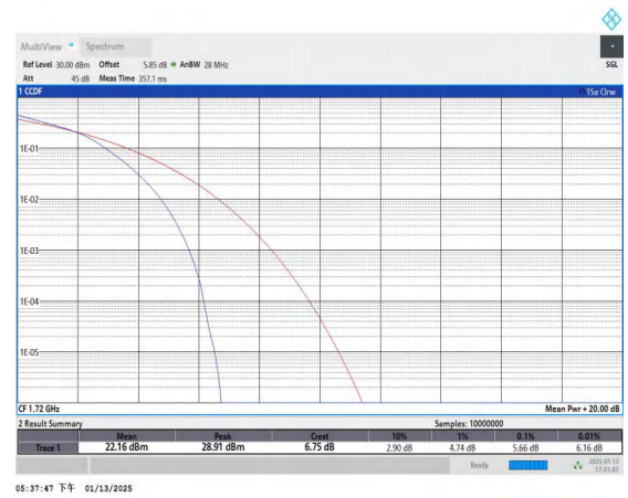
Band4-20MHz-16QAM-20050-100RB#0-PASS
