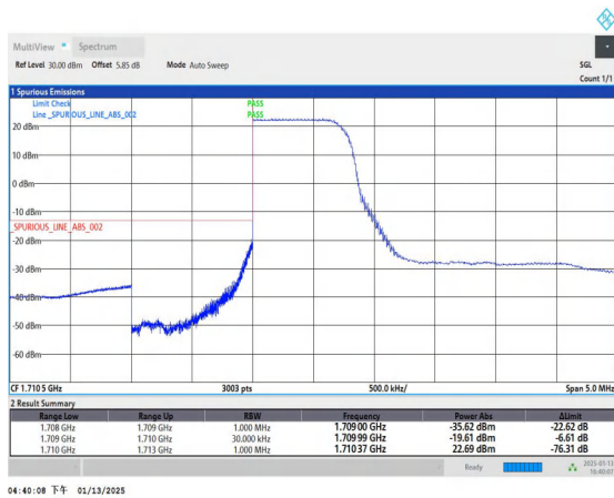
Band4_3MHz_16QAM_19965_1RB#0
