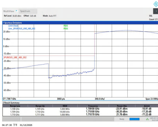
Band4_1.4MHz_QPSK_19957_6RB#0
