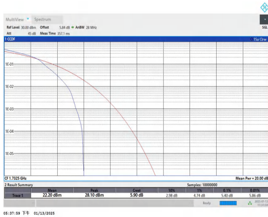
Band4-20MHz-16QAM-20175-1RB#0-PASS
