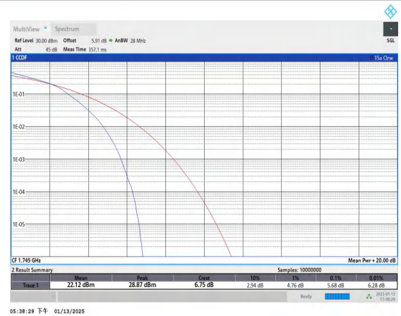
Band4-20MHz-16QAM-20300-100RB#0-PASS
