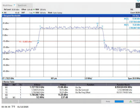
Band4-10MHz-16QAM-20175-50RB#0-PASS
