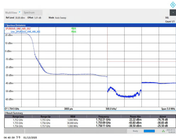
Band4_3MHz_QPSK_20385_1RB#0
