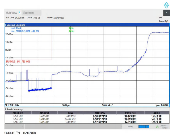
Band4_5MHz_16QAM_19975_1RB#24
