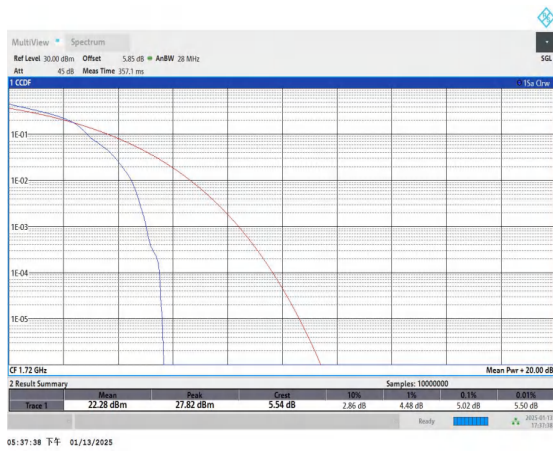
Band4-20MHz-16QAM-20050-1RB#0-PASS
