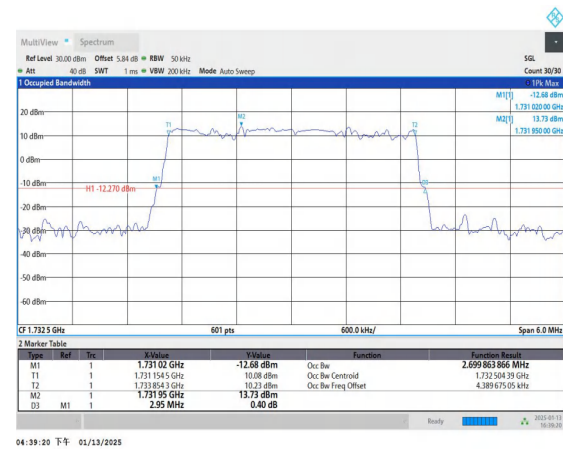
Band4-3MHz-QPSK-20175-15RB#0-PASS
