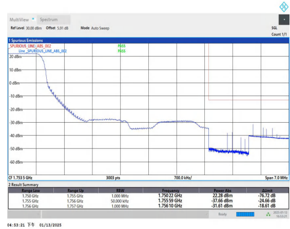
Band4_5MHz_QPSK_20375_1RB#0
