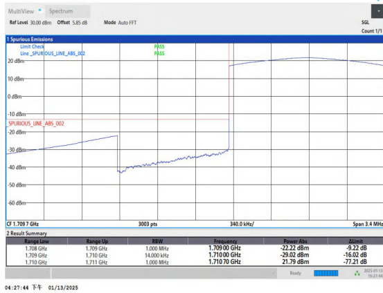
Band4_1.4MHz_16QAM_19957_6RB#0
