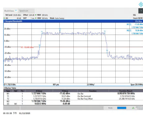
Band4-10MHz-QPSK-20175-50RB#0-PASS
