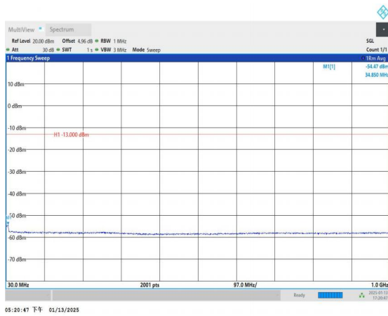
Band4_15MHz_QPSK_20325_1RB#0_30~1000_30~1000
