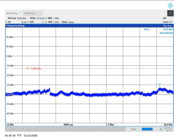
Band4_5MHz_16QAM_20375_1RB#0_3000~20000_3000~2000 00
