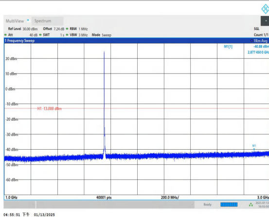
Band4_5MHz_16QAM_20375_1RB#0_1000~3000_1000~3000
