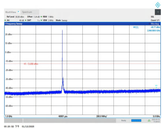
Band4_15MHz_QPSK_20325_1RB#0_1000~3000_1000~3000
