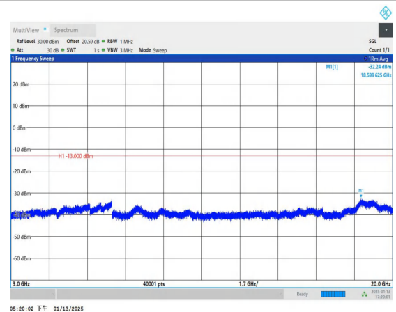
Band4_15MHz_16QAM_20025_1RB#0_3000~20000_3000~2000
