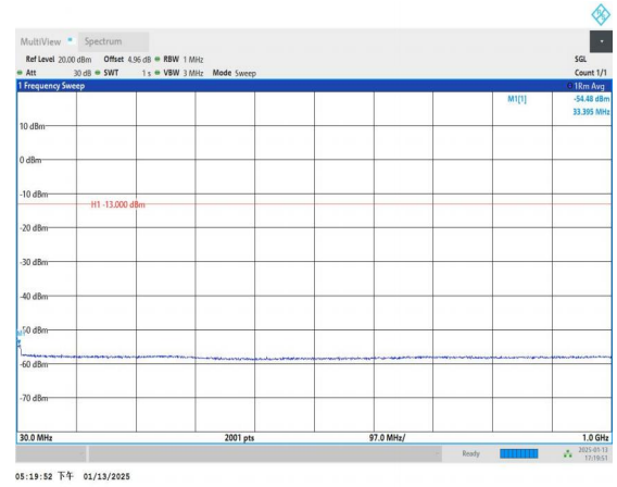
Band4_15MHz_16QAM_20025_1RB#0_30~1000_30~1000
