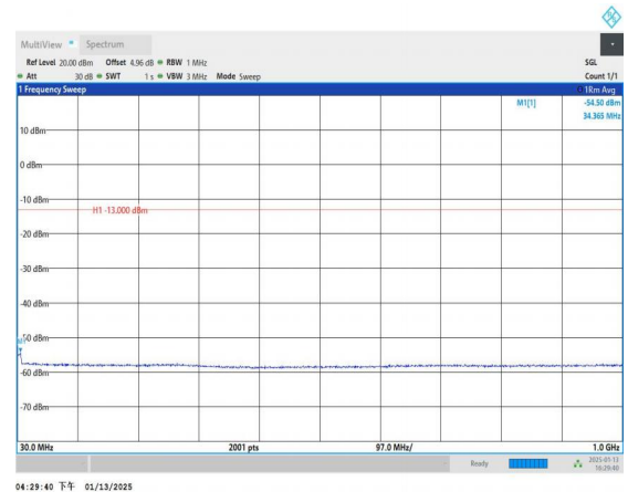
Band4_1.4MHz_16QAM_19957_1RB#0_30~1000_30~1000
