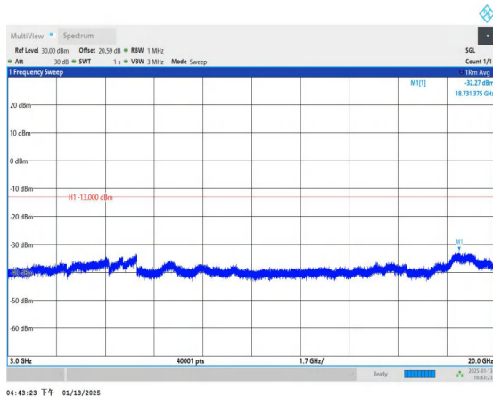
Band4_3MHz_QPSK_20385_1RB#0_3000~20000_3000~20000
