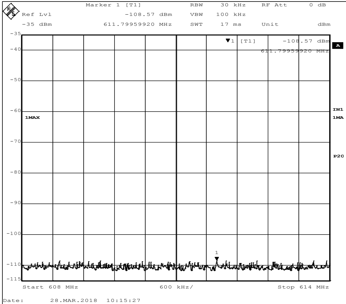
Figure 18 - Band-edge Measurement, Low Channel, Restricted Frequency, Hopping The plot shows an uncorrected measurement, used for relative measurements only.
