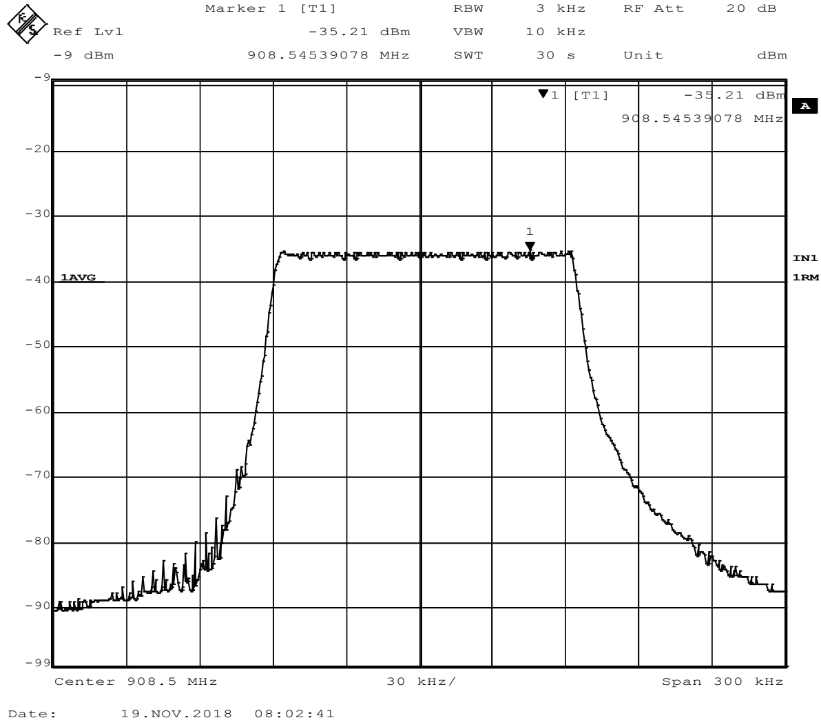
Figure 25 - Power Spectral Density, Mid Channel
