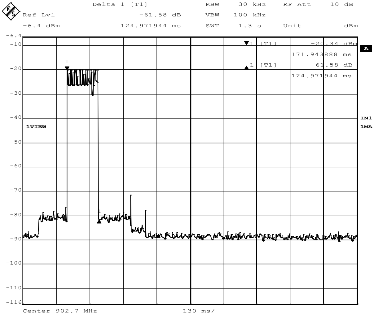
Figure 29 – Time of Occupancy, On Time, 124.97 ms
