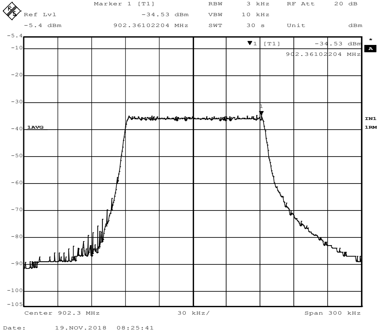
Figure 24 - Power Spectral Density, Low Channel
