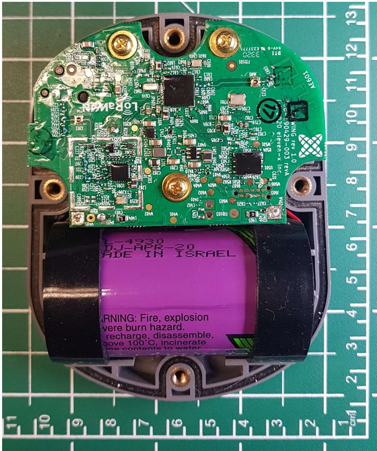
PCB with battery in enclosure bottom
