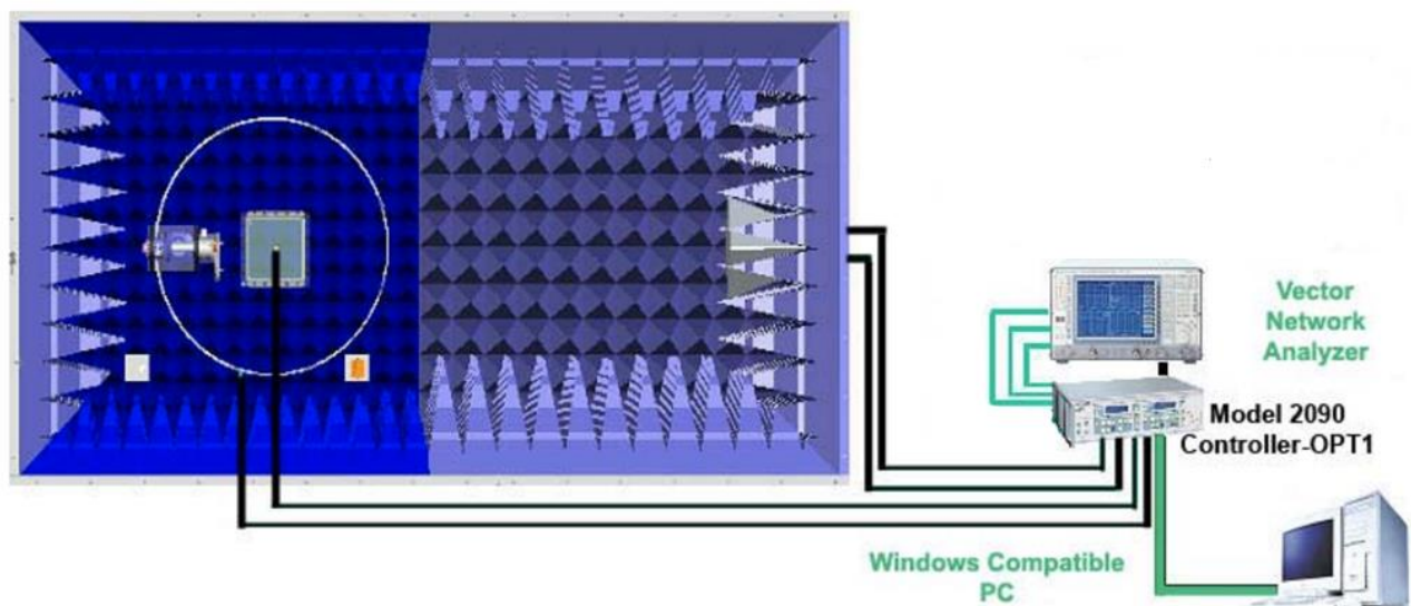
Figure 1: Measurement system with 3164-04 Horn Antenna
