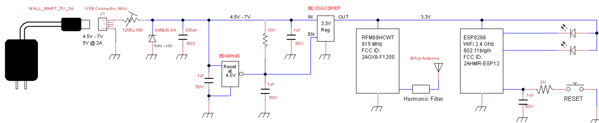
Figure 3. Flume Bridge Block Diagram.
