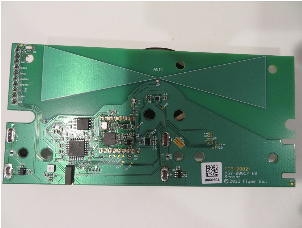
SENSOR BOTTOM
