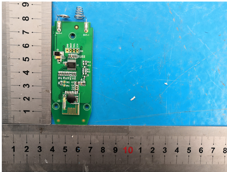
EUT –Bottom Chip View
