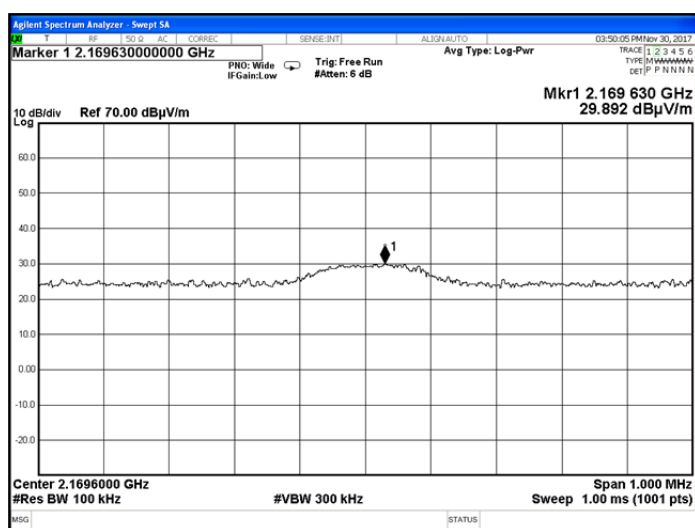
Plot 7.2.14 Radiated emission measurements at the 5th harmonic frequency
