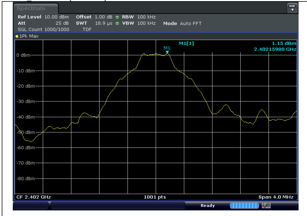
GFSK 2 402 MHz(reference)
