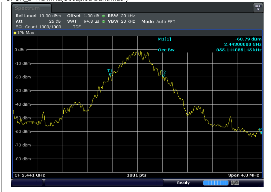
GFSK 2 441 MHz(Occupied Bandwidth)
