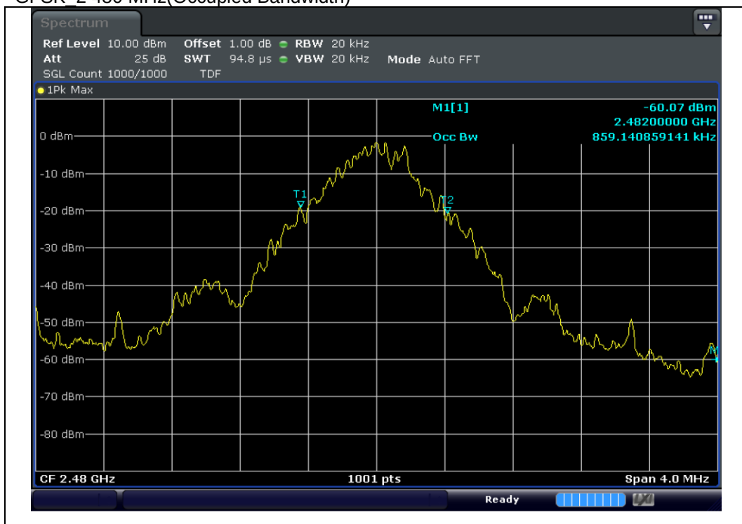
GFSK 2 480 MHz(Occupied Bandwidth)
