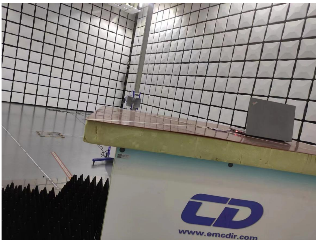
>1GHz
