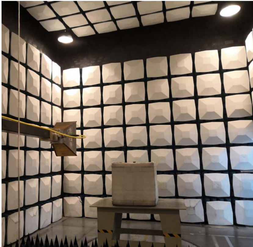
Radiated Emission Above 1GHz View
